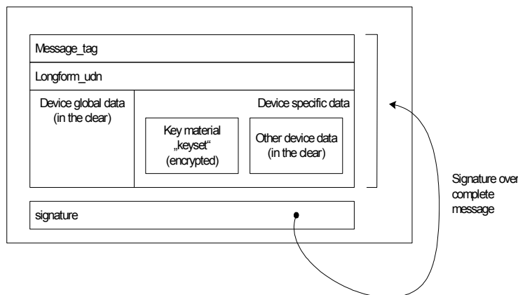
Figure 17: domain_registration_response() message
