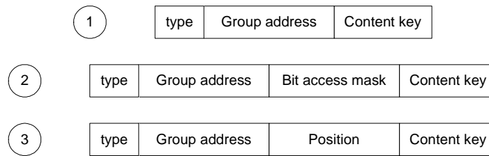
Figure 31: Addressing modes
