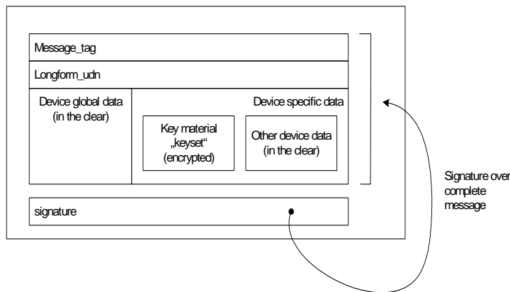
Figure 9: device_registration_response() message
