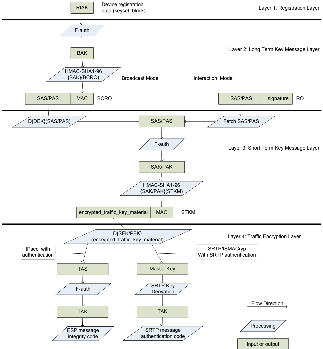
Figure 3: Authentication hierarchy
