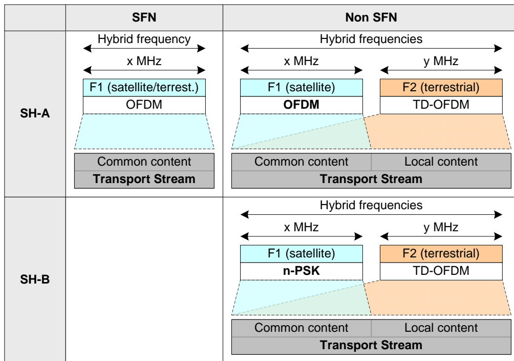
Figure 1: DVB-SH system configurations
