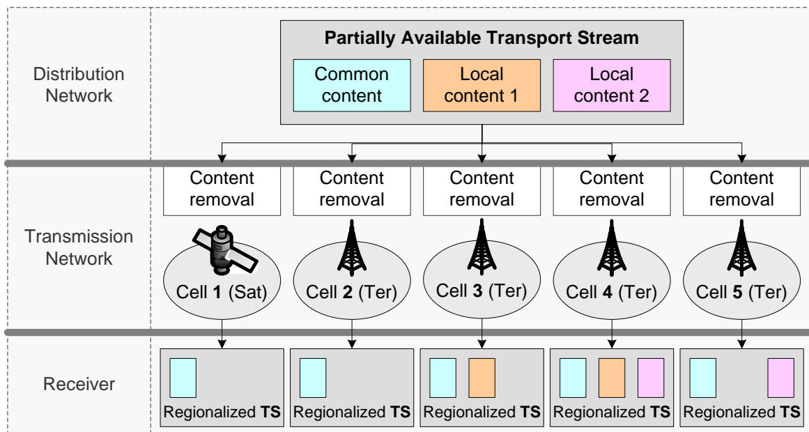
Figure 2: Local content insertion via content removal
