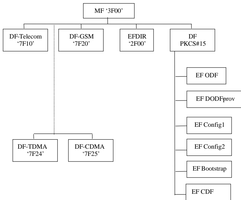
Figure 3: File structure for WAP data on RUIM smart card or 2G UICC
