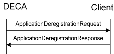
Figure 57: DCD-Enabled Client Application Deregistration with DCD Client
