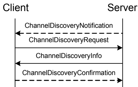
Figure 34: Channel Discovery Notification / Pull Transactions
