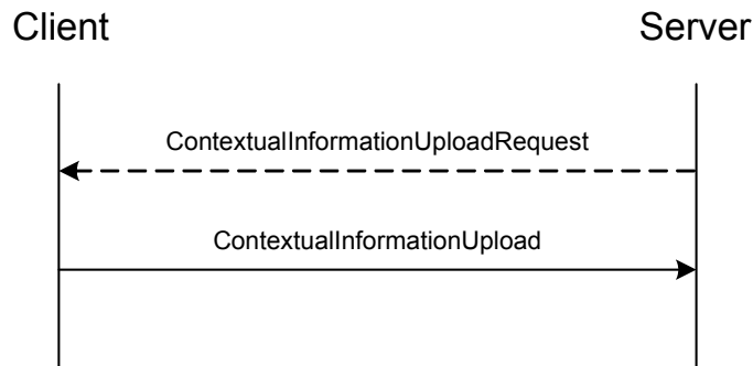
Figure 27: Contextual Information Upload
