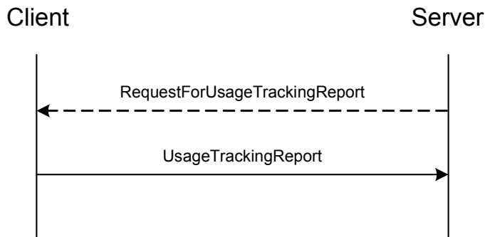
Figure 28: Usage Tracking Report transaction
