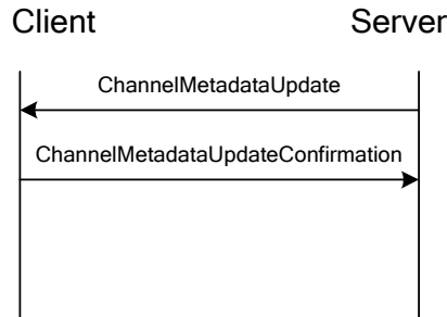
Figure 40: Channel Metadata Update
