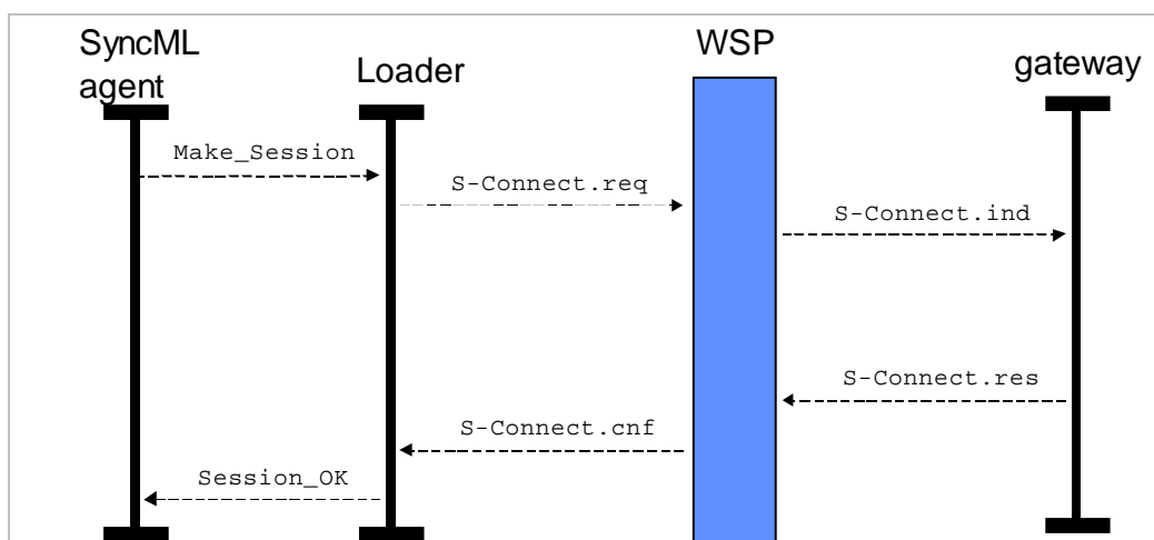
Figure 1: Session Establishment
