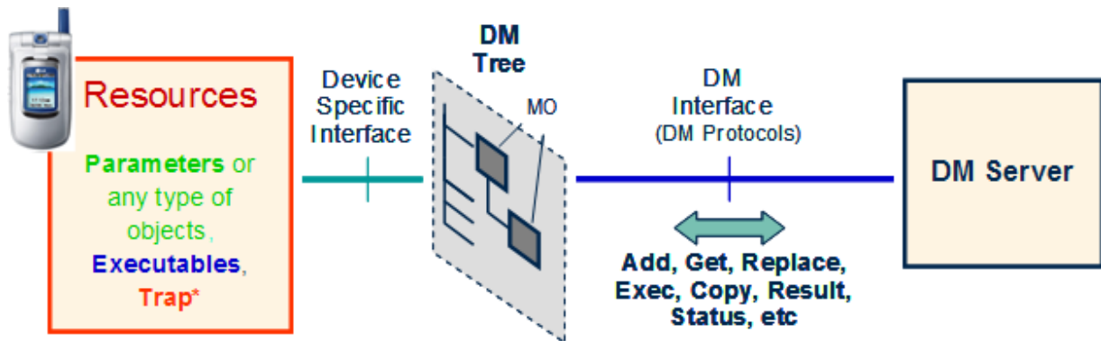
Figure 1: Device management
