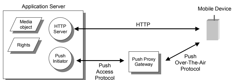
Figure 3. An example architecture for separate delivery
