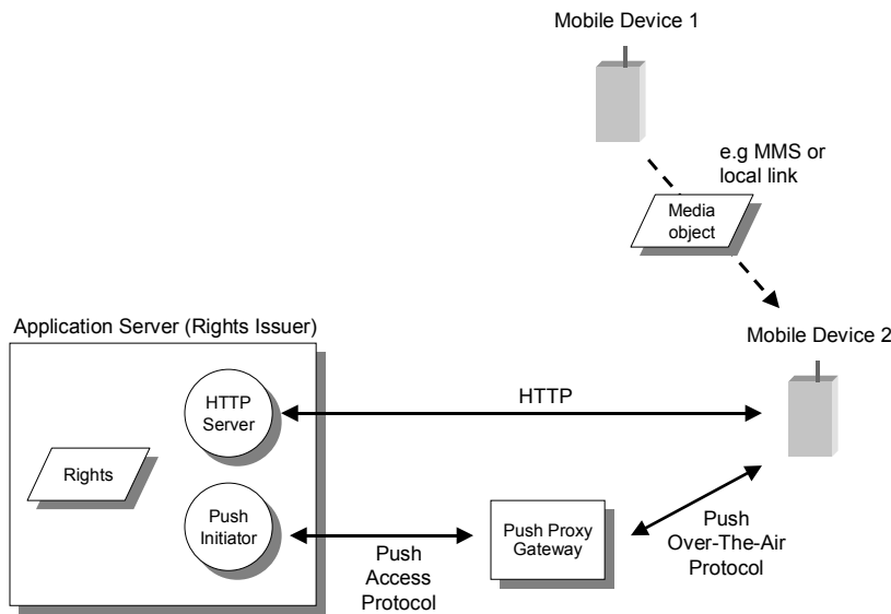
Figure 4 – An example architecture for Superdistribution
