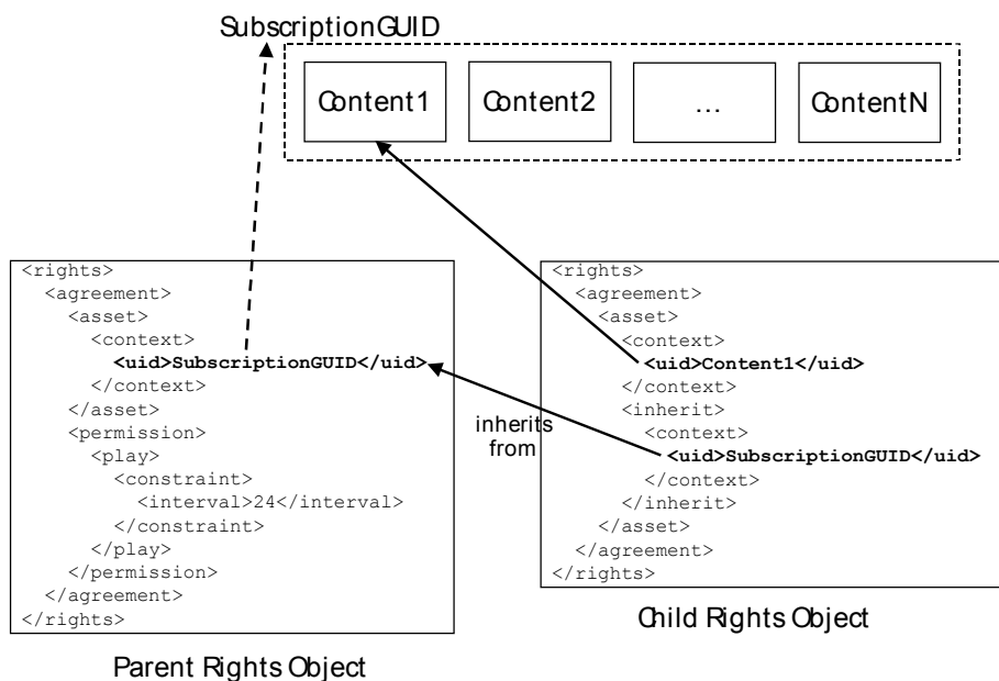
Figure 5.1. Inheritance.
