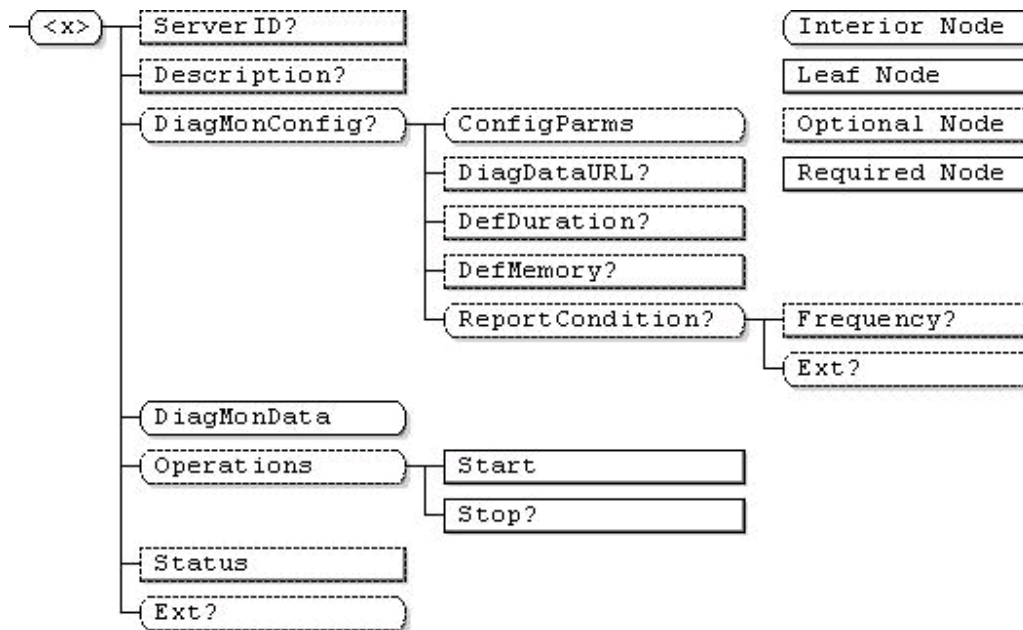
Figure 1: Diagnostics and Monitoring Management Object
