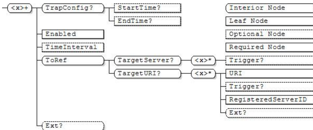
Figure 1: DiagMon Trap Management Object
