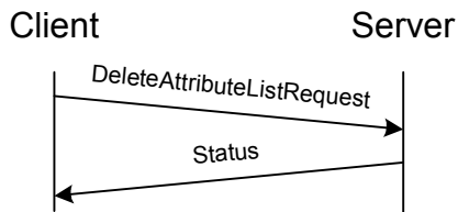
Figure 22. Delete attribute list transaction
