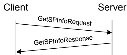
Figure 7. Get Service Provider Info transaction
