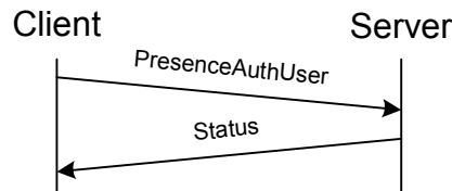
Figure 30. Reactive presence authorization of user transaction
