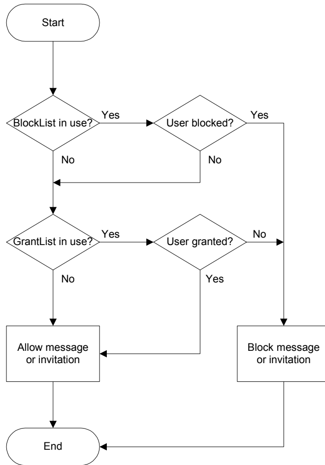
Figure 43. Blocking decision-tree
