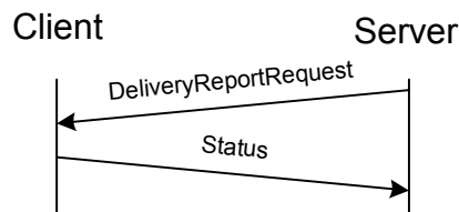
Figure 41. Delivery Status Report Transaction
