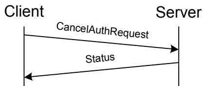
Figure 31. Cancel presence authorization transaction
