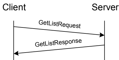
Figure 17. Get list of contact list IDs transaction
