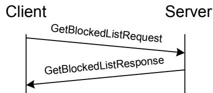
Figure 44. Get list of blocked entities transaction
