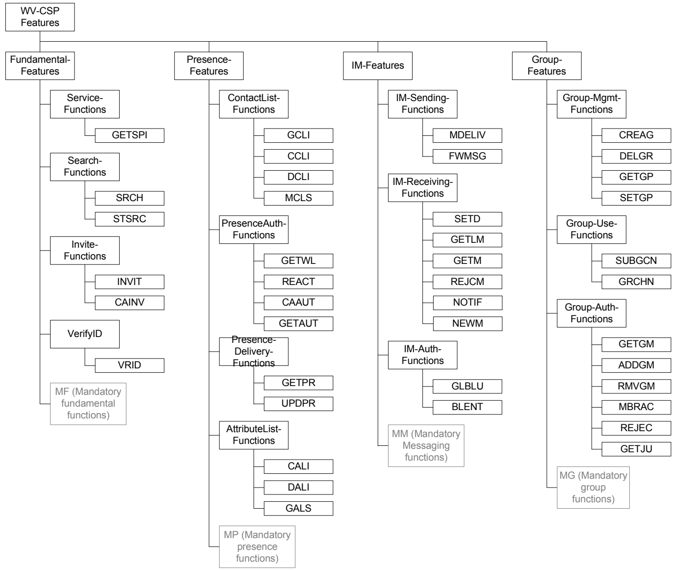
Figure 9. The service tree
