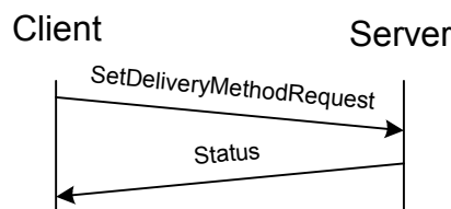
Figure 35. Set Delivery Method transaction
