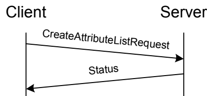
Figure 21. Create attribute list transaction
