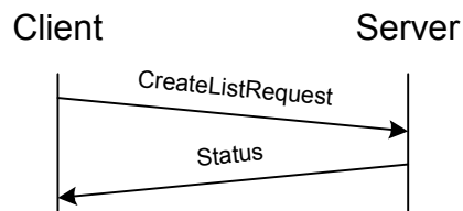
Figure 18. Create contact list transaction
