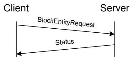
Figure 45. Block/unblock entities transactions
