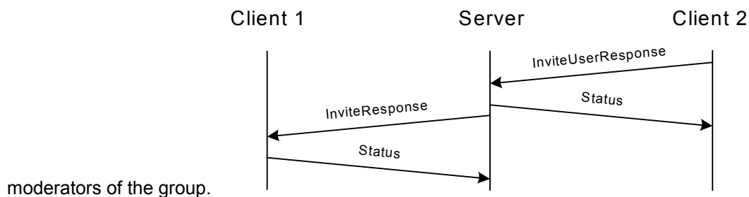
Figure 14. Invited users’ response
