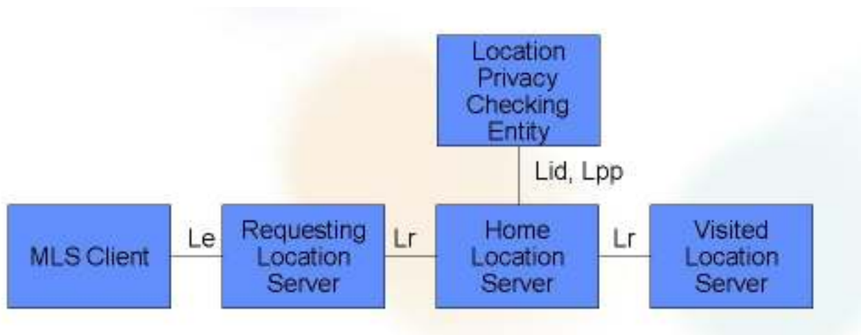
Figure 1: Architectural diagram of MLS
