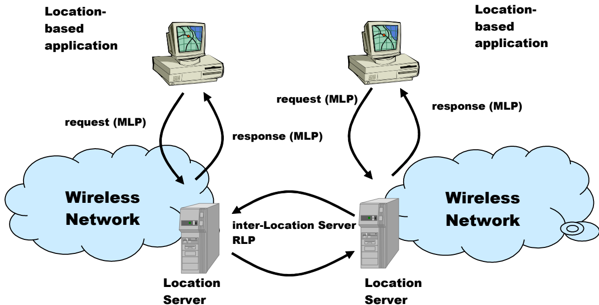
Figure 1: RLP Overview
