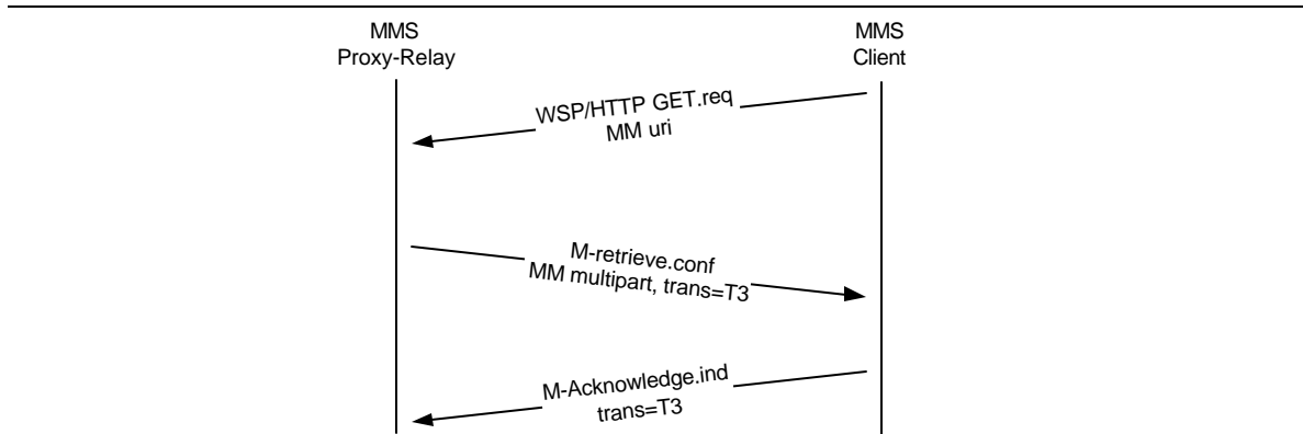
Figure 12. Example MMS Retrieval Transaction with Acknowledgement
