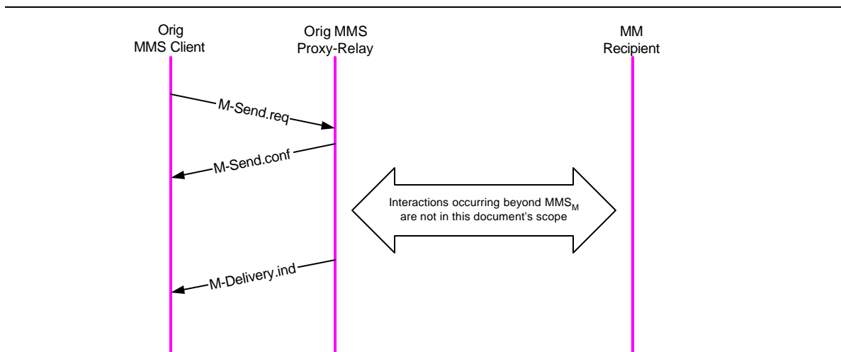
Figure 4. Example MMS_M Transaction Flow – Sending
