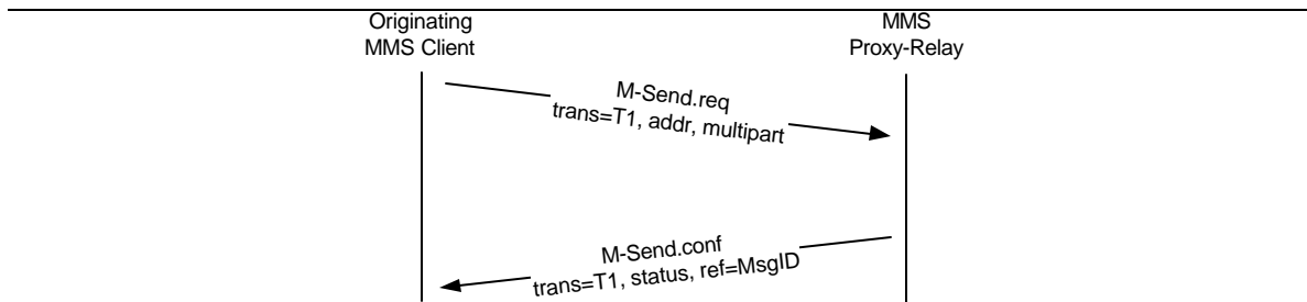
Figure 9. Example MMS Send Transaction
