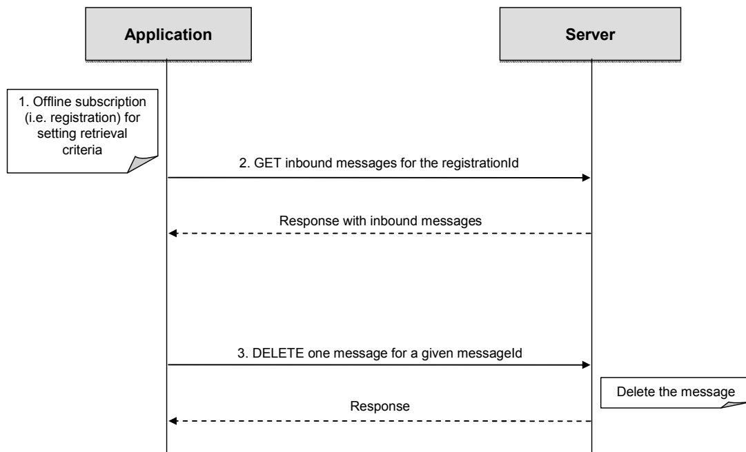
Figure 4: Inbound SMS message delivery (polling mode)
