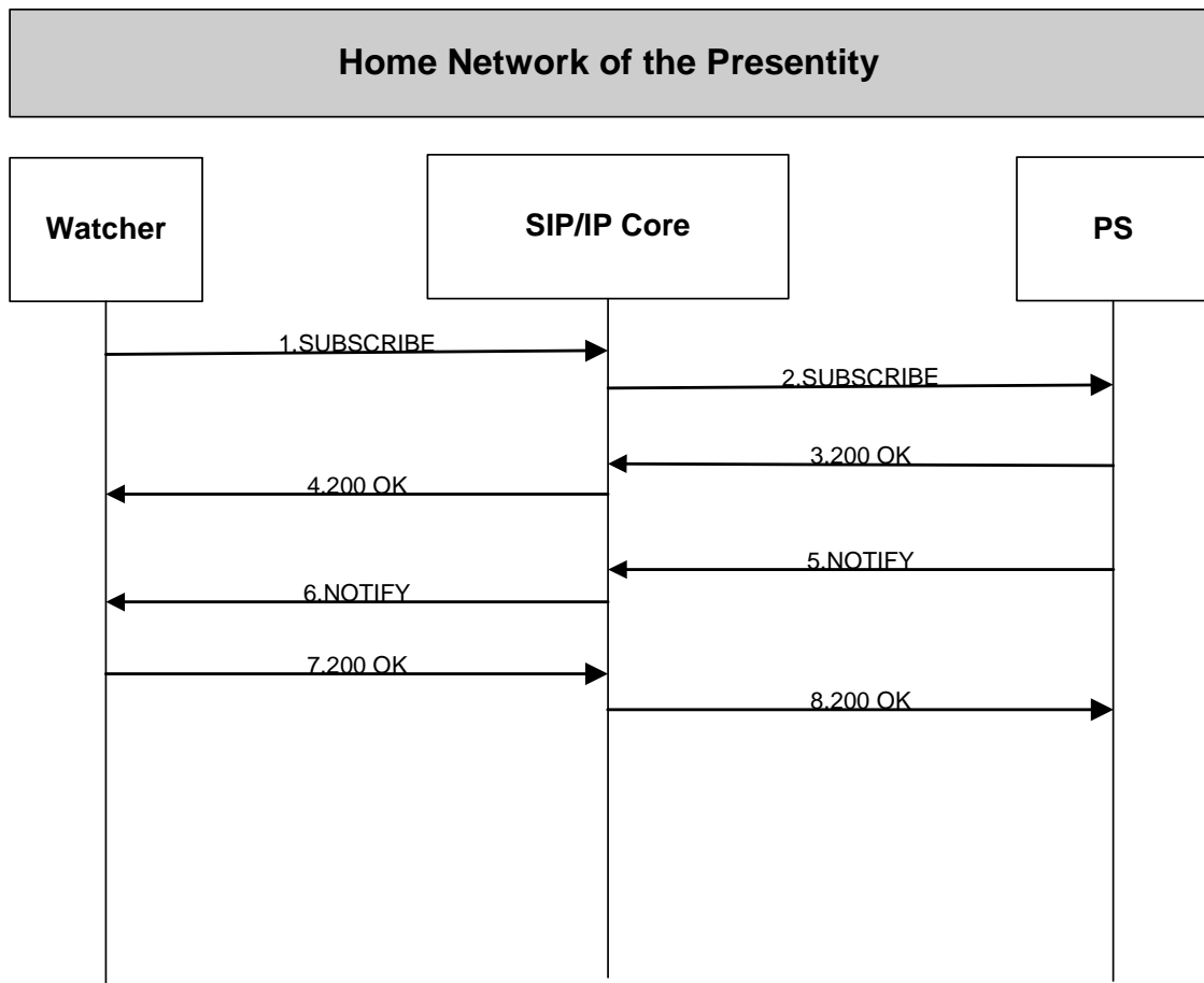
Figure 17 - Subscription Filters
