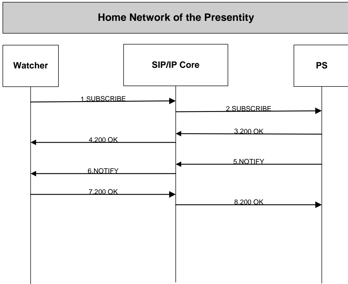
Figure 16- Polite Blocking
