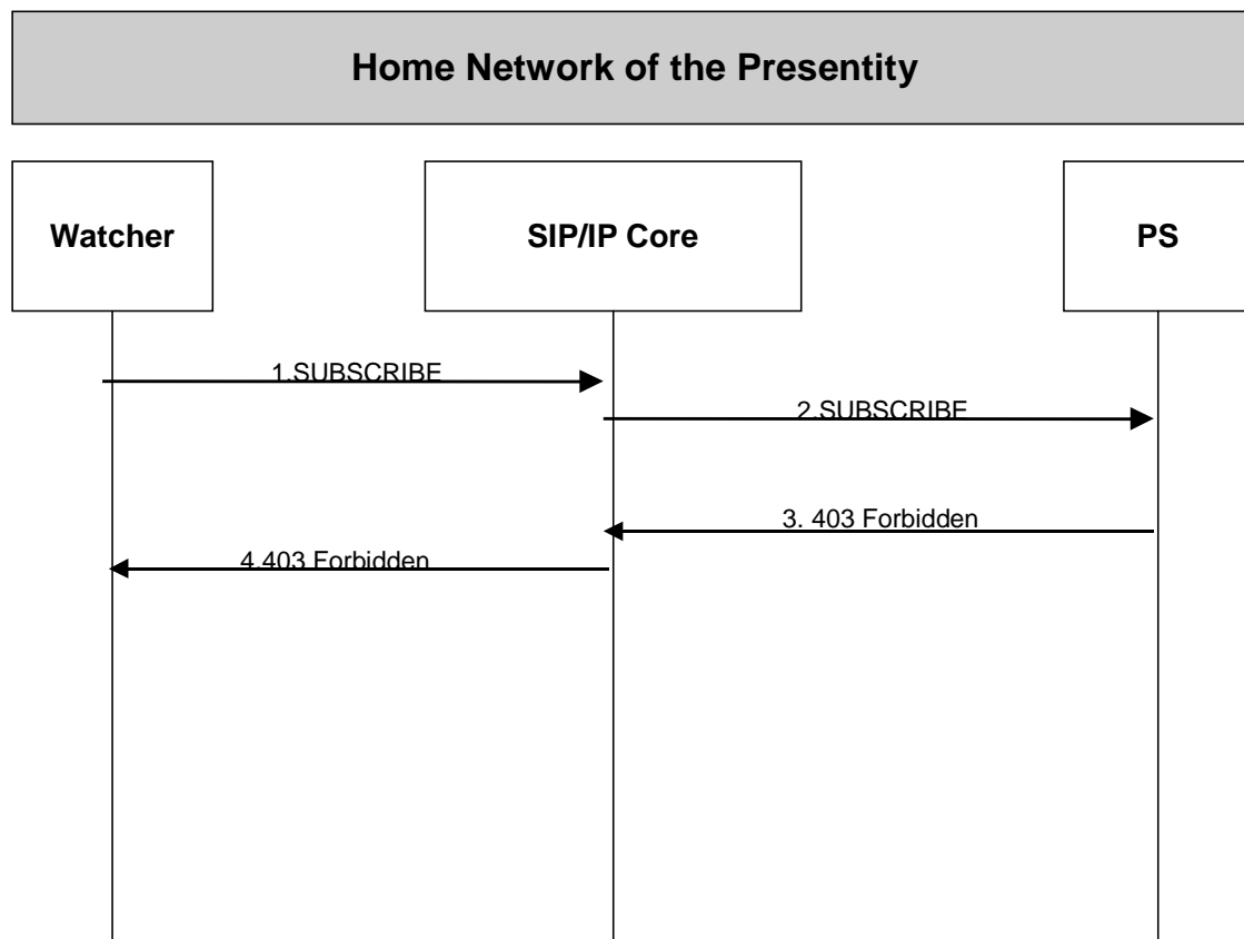
Figure 15 - Blocking
