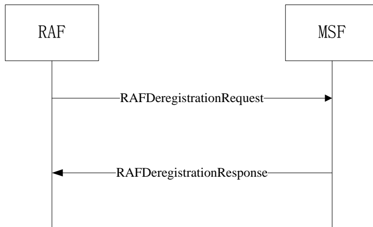
Figure 13: RCC Deregistration messages exchange
