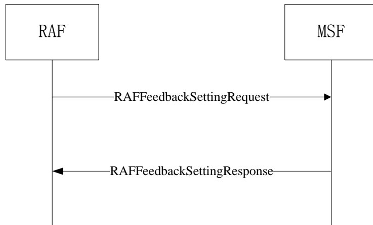
Figure 25: Feedback setting messages exchange
