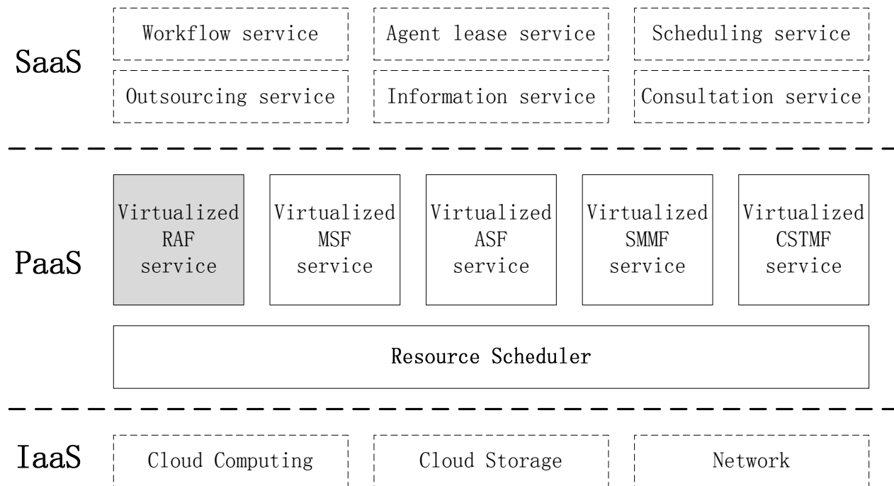
Figure 36: Virtualized RCC framework
