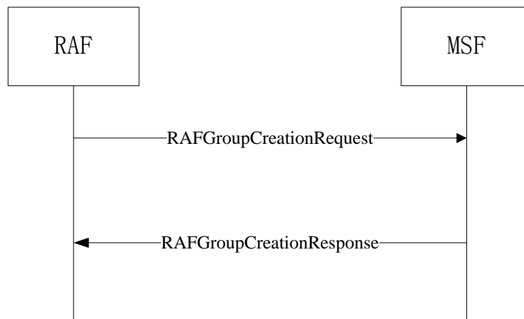
Figure 17: RCC agent group creation messages exchange
