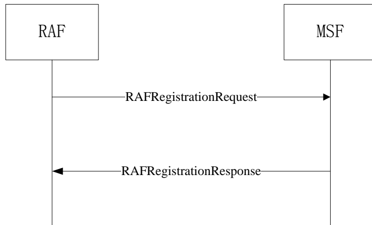
Figure 12: RCC Registration messages exchange
