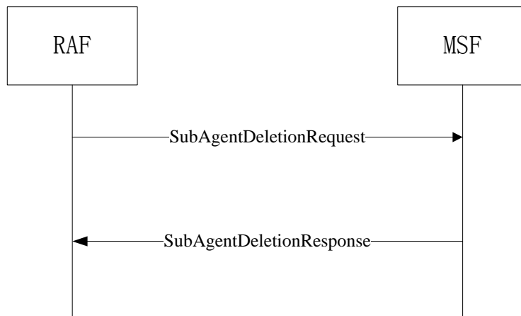
Figure 21: RCC sub-agent deletion messages exchange
