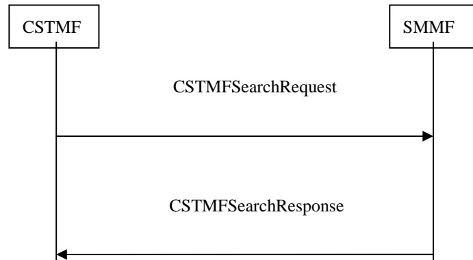
Figure 29: CSTMF social media search messages exchange
