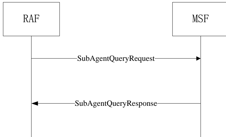
Figure 22: RCC sub-agent query messages exchange
