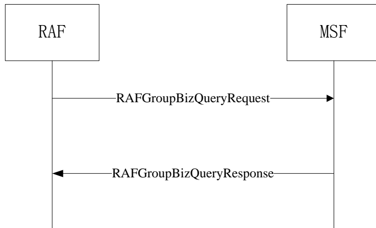
Figure 23: RCC agent group busyness query messages exchange
