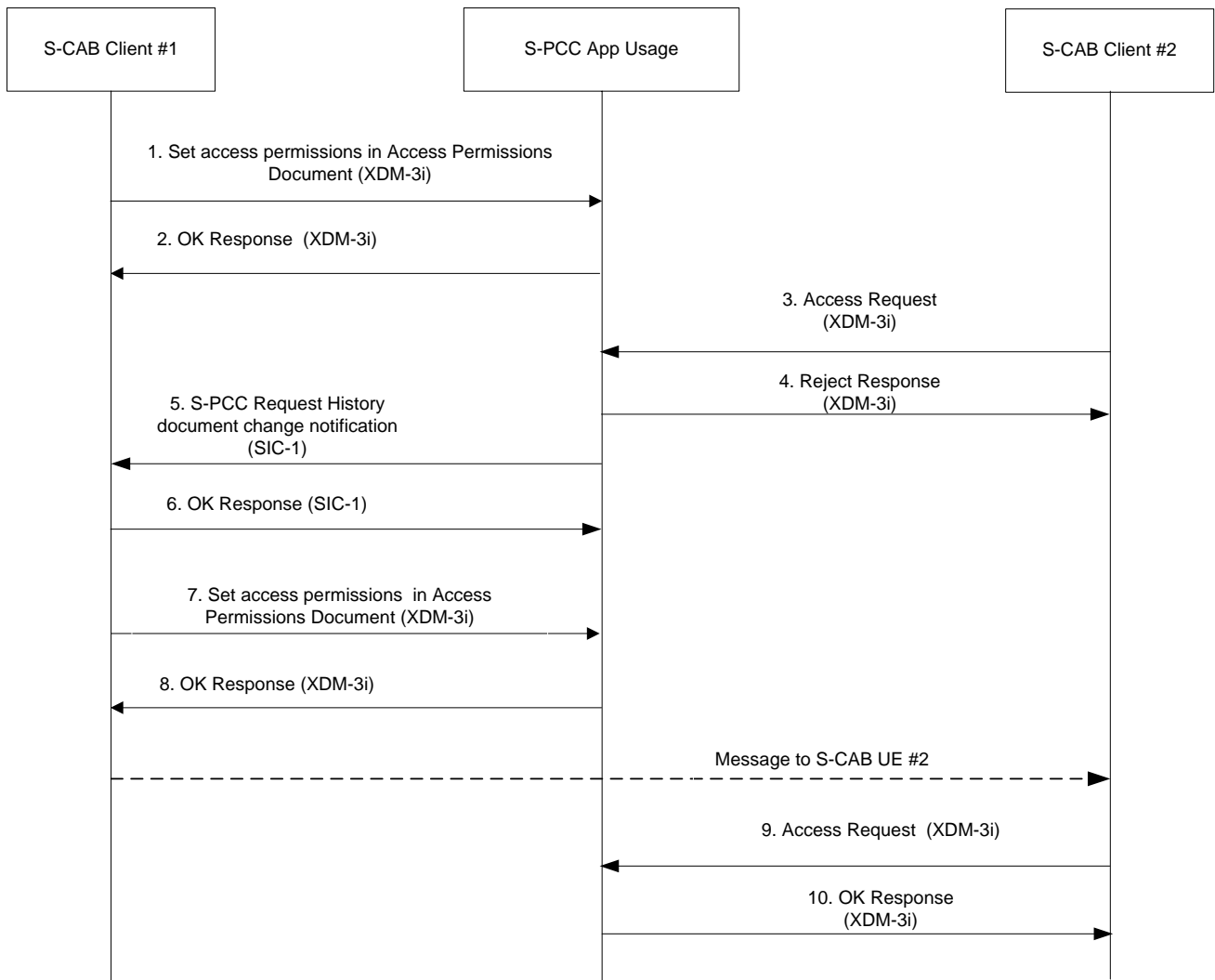
Figure 8: Reactive authorization
