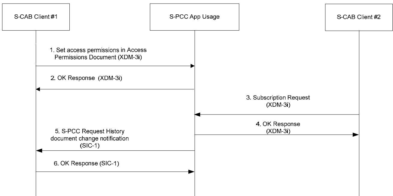
Figure 9: Automatic authorization
