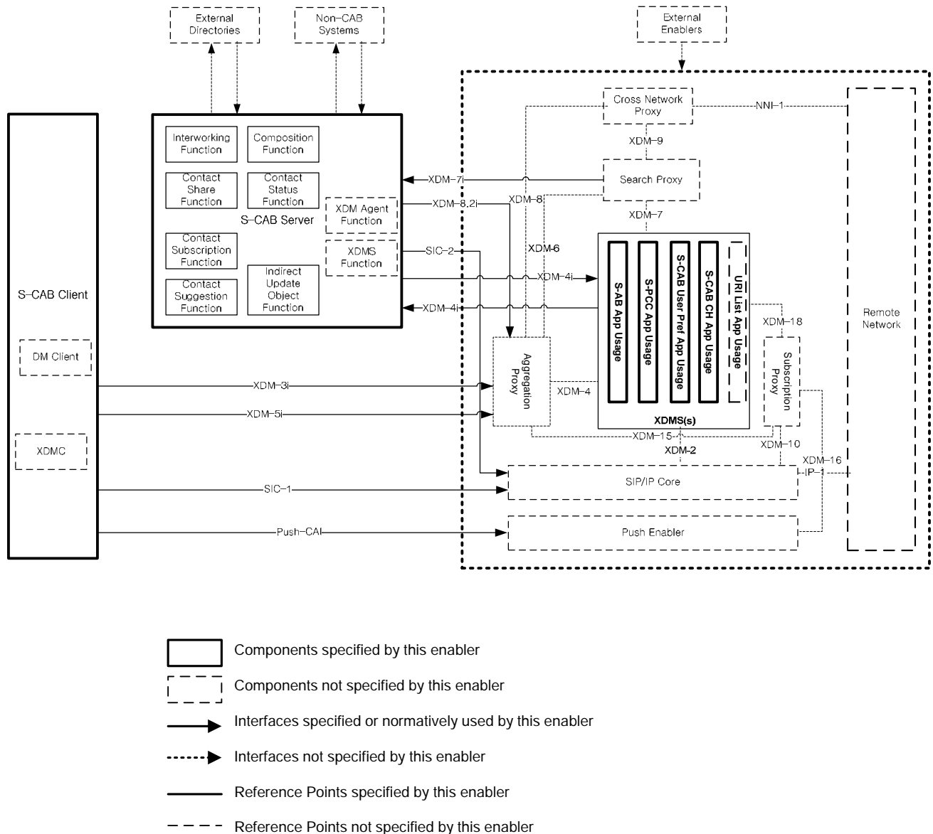
Figure 22: S-CAB Architecture Showing XDM Components (Informative)
