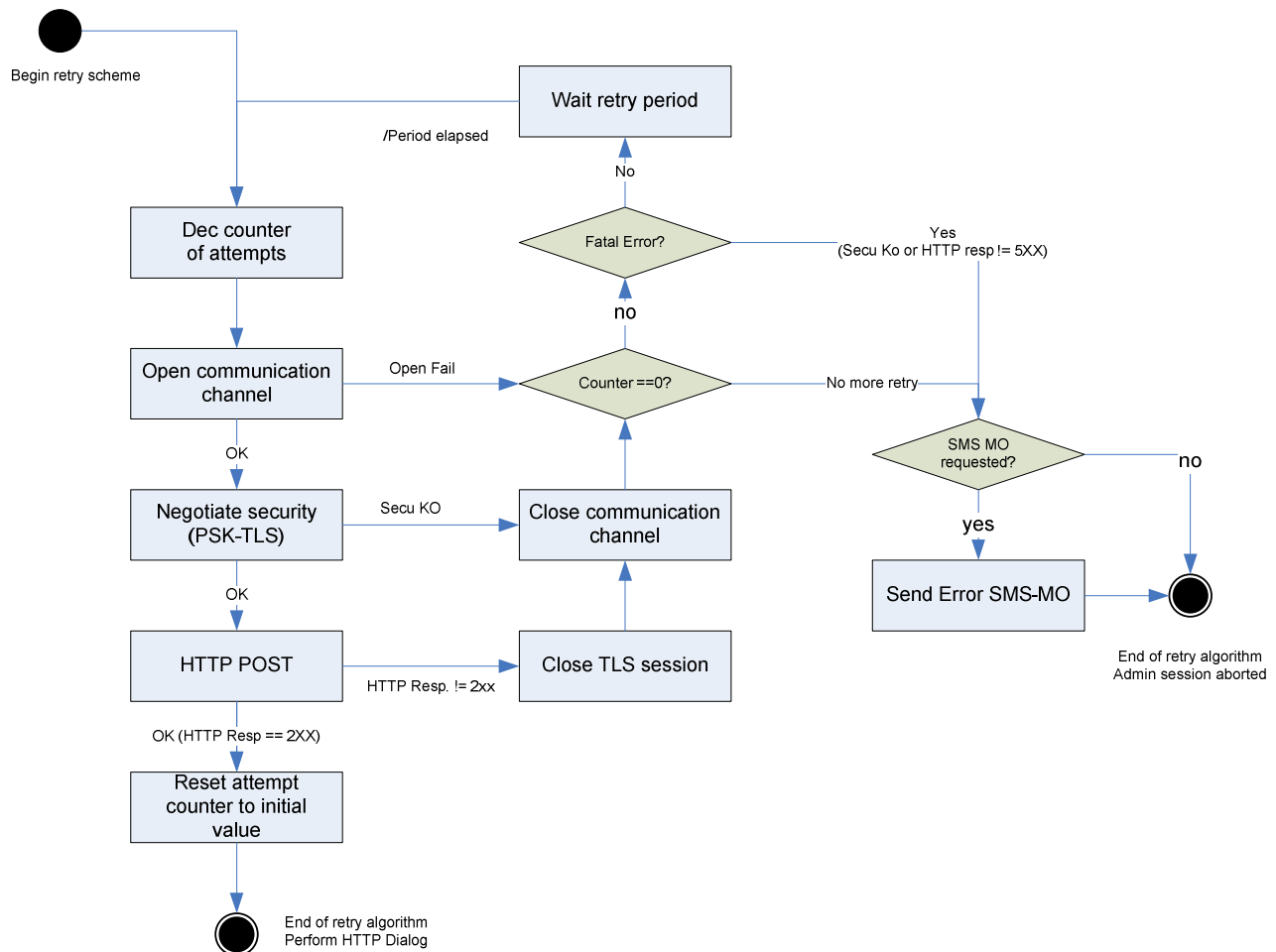
Figure 3: Retry algorithm
