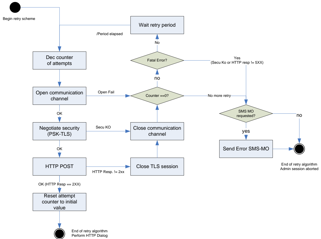
Figure 4: Retry algorithm
