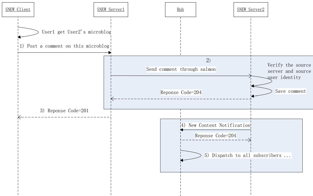
Figure 7: Example flow of cross domain reactions
