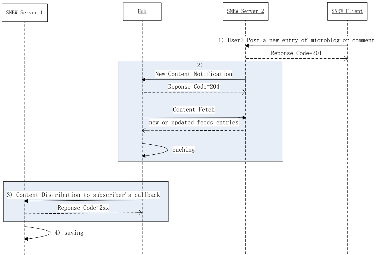
Figure 6: Example flow of cross domain activities dispatching
