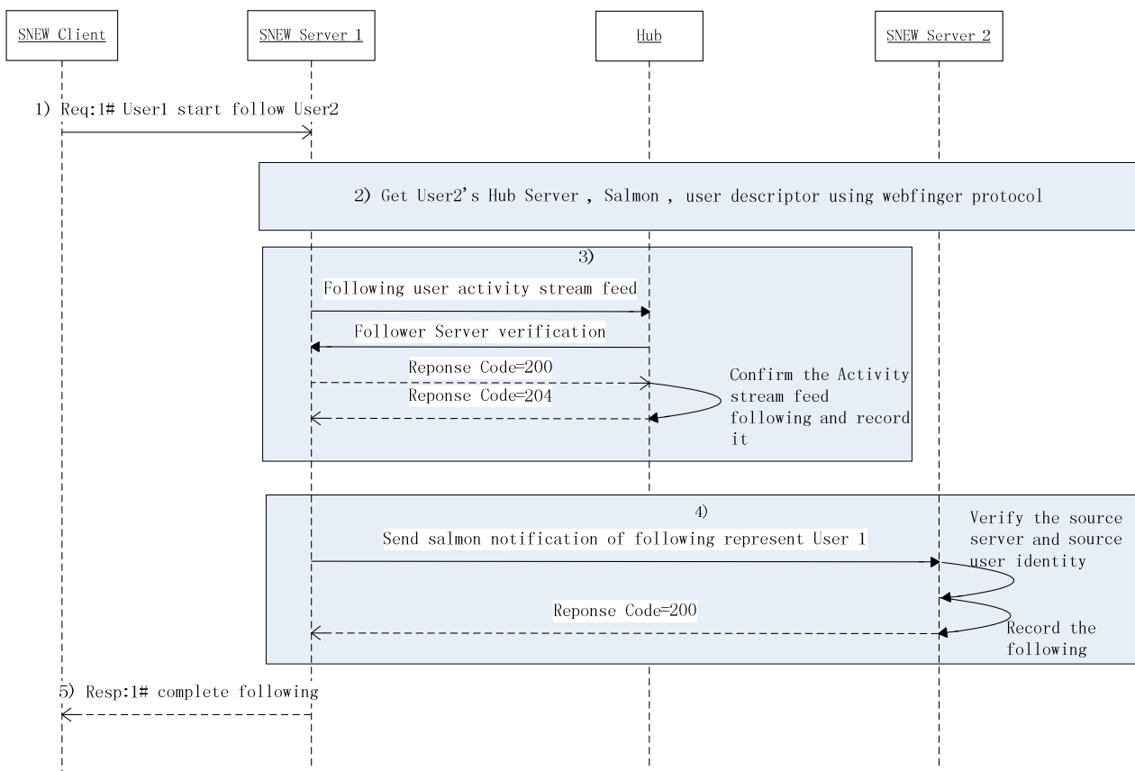
Figure 5: Example flow of cross domain subscription
