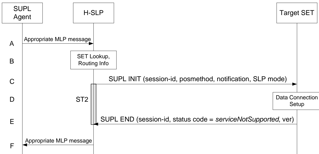
Figure 45: Network Initiated, SET does not support the service requested in SUPL INIT .....127
