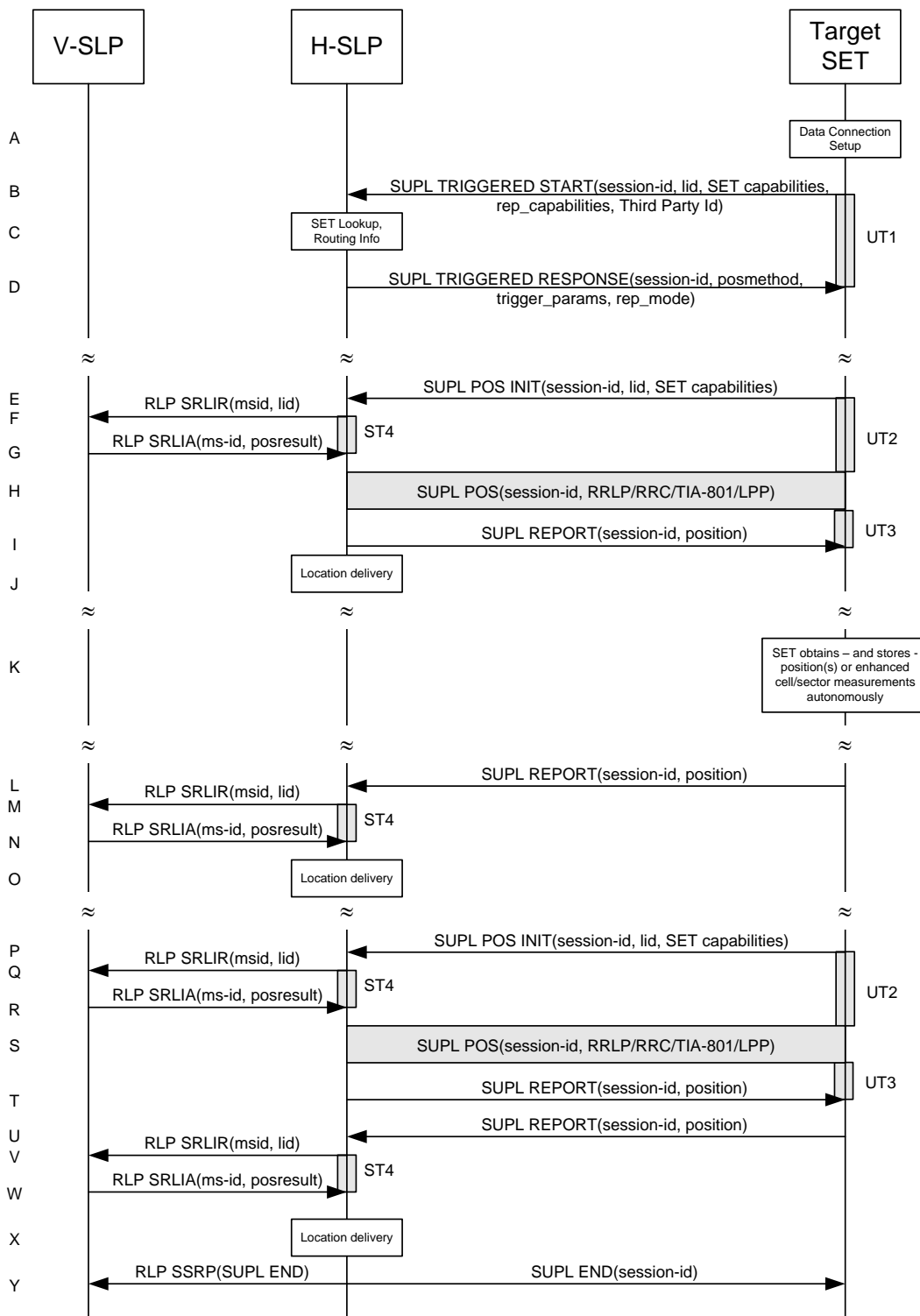
Figure 67: SET Initiated Periodic Location Request with transfer of the position result to 3 rd party – roaming with H-SLP Positioning – proxy mode
