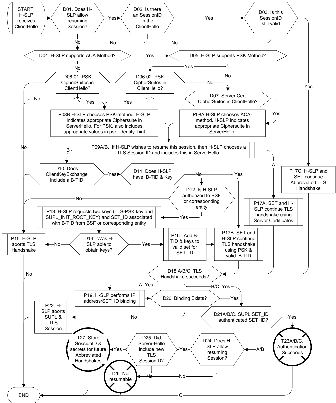
Figure 106: The generic version of the Security Negotiation Model for the H-SLP.
