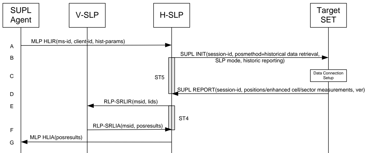
Figure 28: Retrieval of historical positions and/or enhanced cell/sector measurements – roaming
