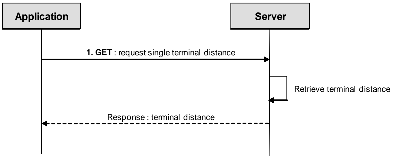
Figure 3 Distance from location query
