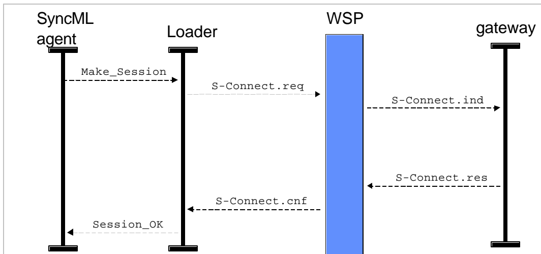
Figure 1 Session Establishment
