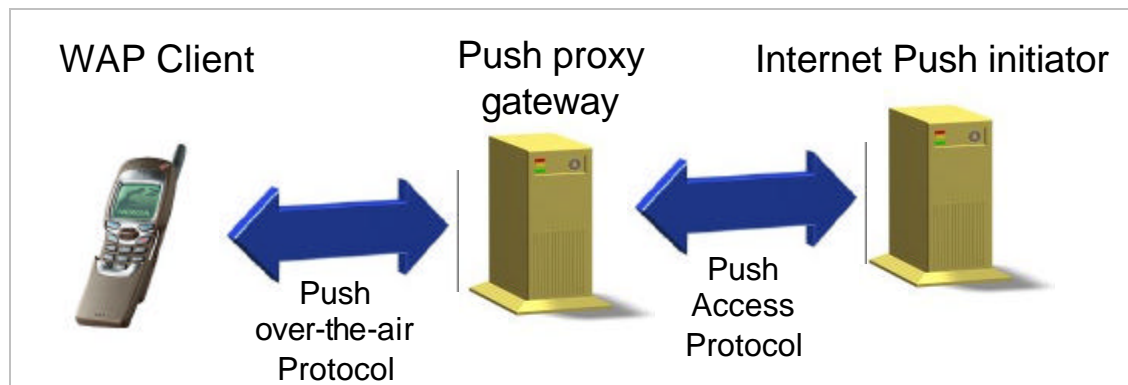
Figure 4 Push Model
