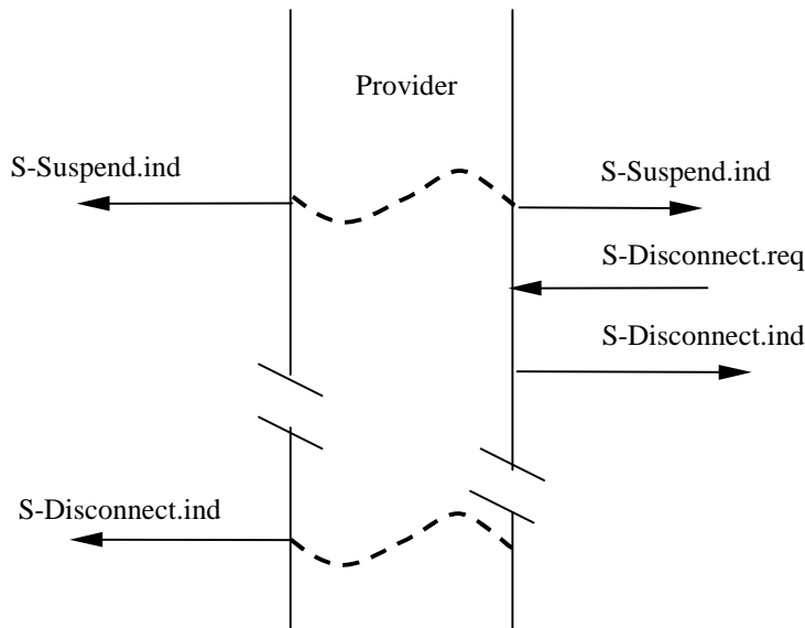
Figure 7: Suspended Session Termination
