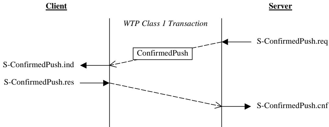
Figure 10. Confirmed Push Invocation
