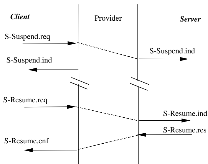
Figure 5: Session Suspension and Resume
