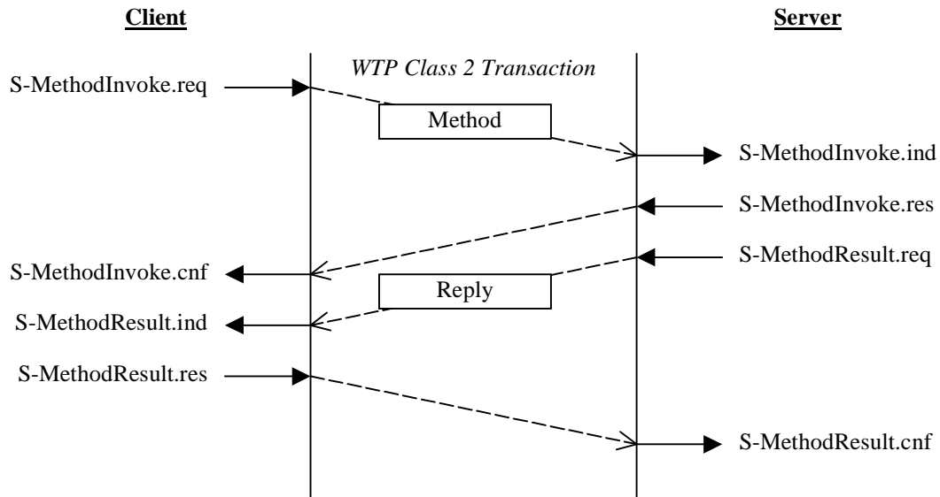
Figure 8. Normal Method Invocation
