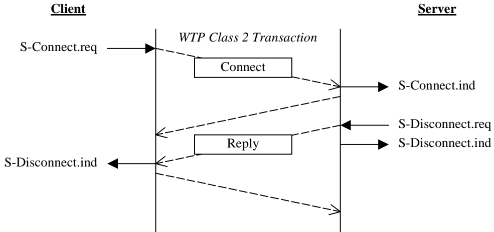
Figure 3. Session Creation with Server Error
