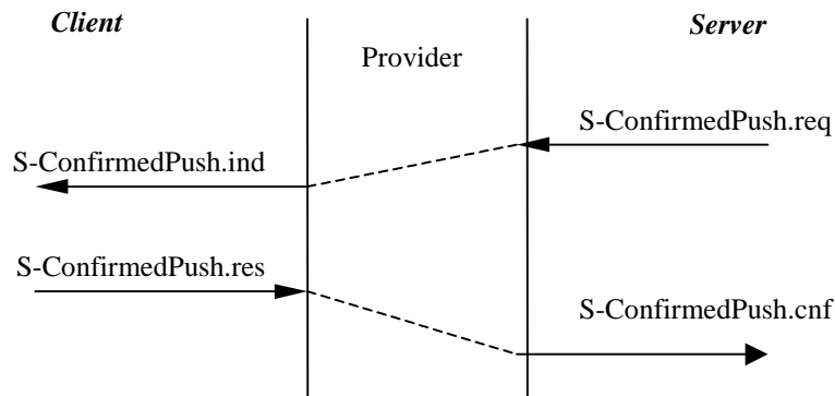
Figure 14: Confirmed Data Push
