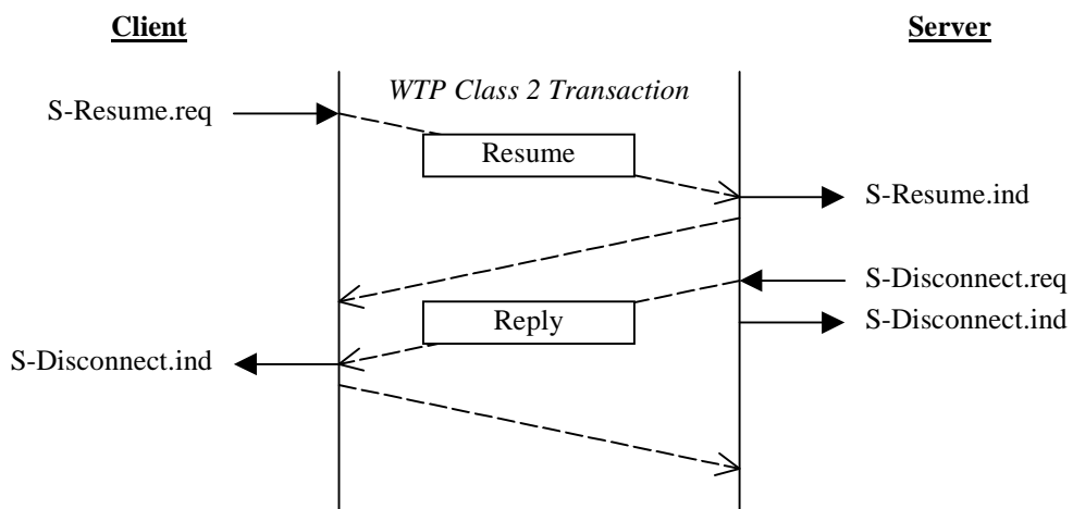
Figure 7. Session Resume with Server Error
