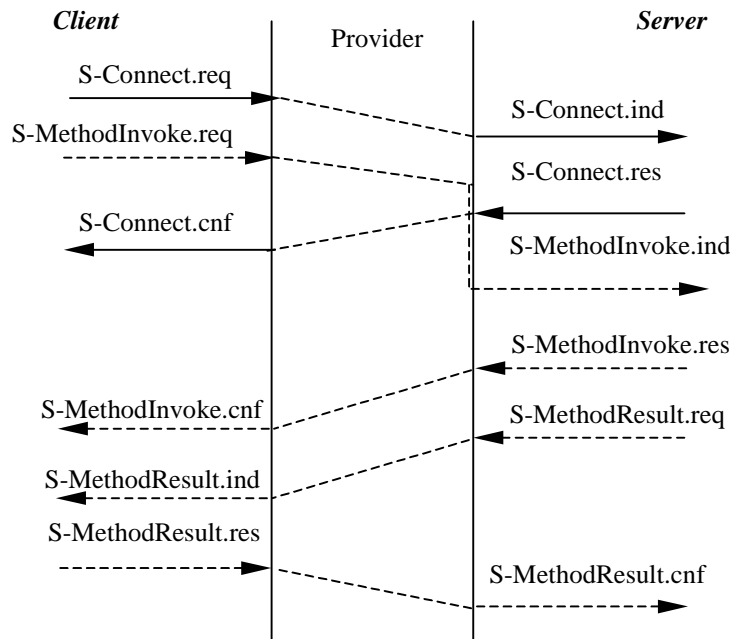
Figure 2: Successful Session Establishment
