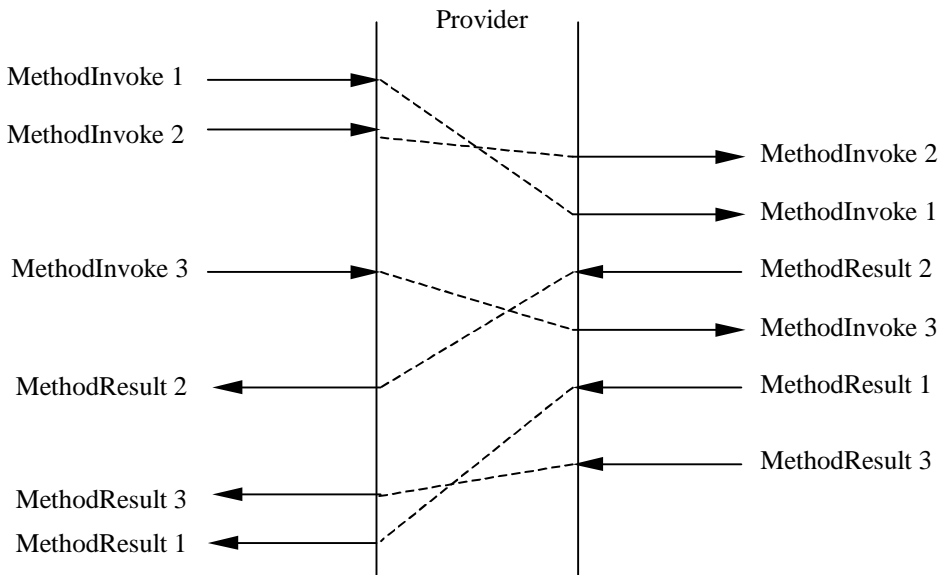
Figure 9: Unordered Asynchronous Requests
