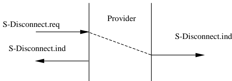
Figure 4: Active Session Termination
