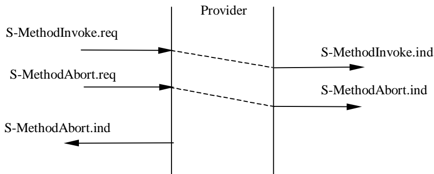
Figure 11: Abort after S-MethodInvoke.indication
