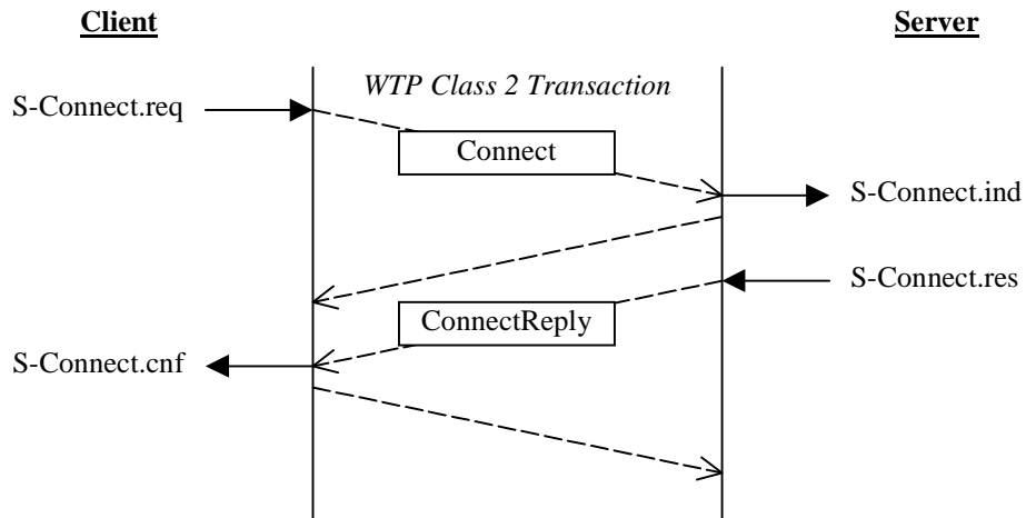
Figure 1. Normal Session Creation
