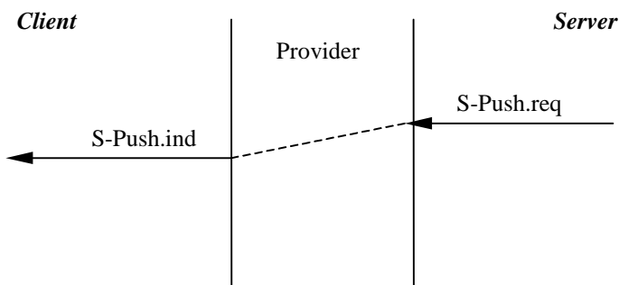
Figure 12: Non-confirmed Data Push
