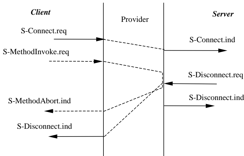
Figure 3: Refused Session Establishment
