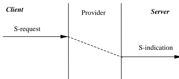
Figure 1: A Non-confirmed Service
