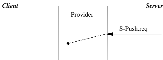
Figure 13: Failed Non-confirmed Data Push
