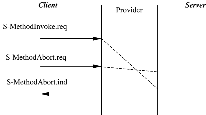
Figure 10: Abort before S-MethodInvoke.indication
