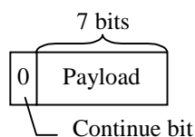
Figure 11. Variable Length Integer Octet
