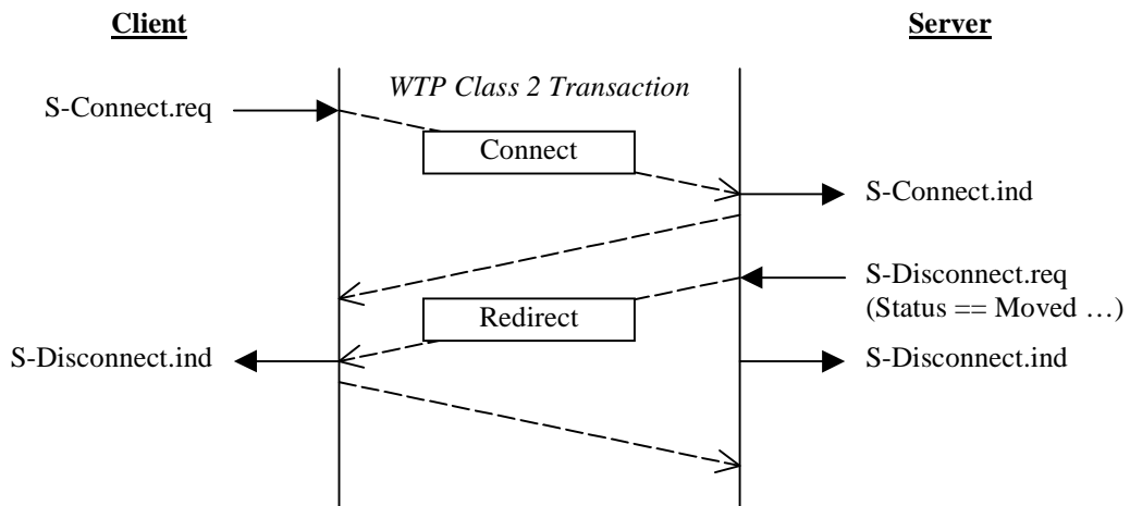
Figure 2. Session Creation with Redirect
