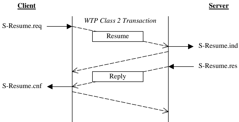
Figure 6. Normal Session Resume
