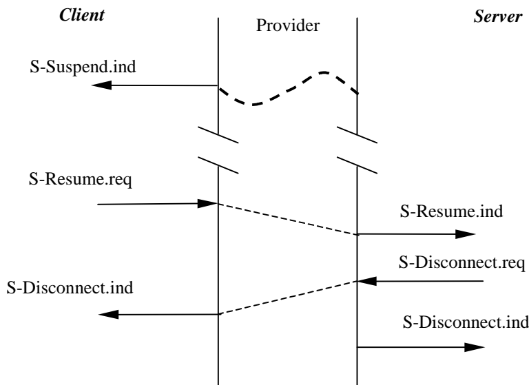
Figure 6: Suspend by Provider and Refused Resume
