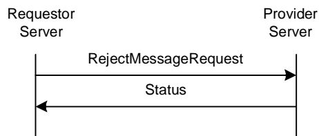
Figure 53. The “RejectMessage” Transaction
