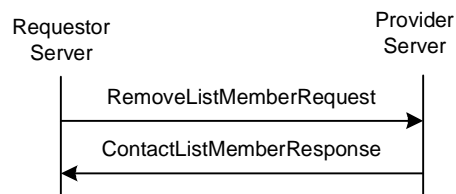
Figure 32. The “RemoveListMember” Transaction
