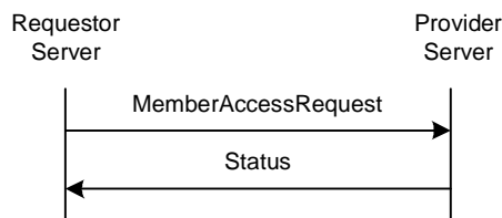
Figure 66. The “MemberAccess” Transaction
