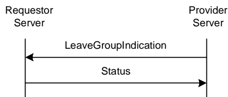
Figure 61. The “ServerInitiatedLeaveGroup” Transaction
