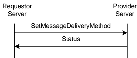
Figure 51. The “SetMessageDeliveryMethod” Transaction
