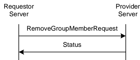
Figure 65. The “RemoveGroupMember” Transaction
