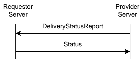
Figure 54. The “NotifyDeliveryStatusReport” Transaction
