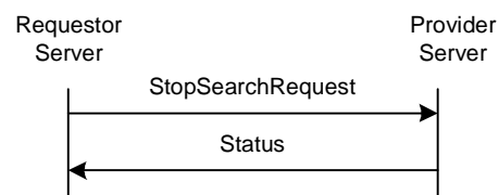
Figure 21. The “StopSearch” Transaction
