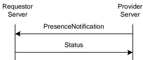
Figure 41. The “PresenceNotification” Transaction
