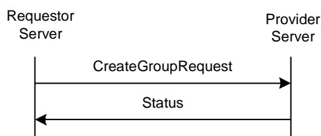
Figure 57. The “CreateGroup” Transaction
