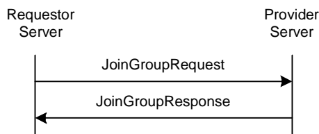
Figure 59. The “JoinGroup” Transaction
