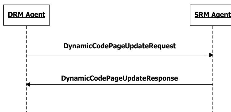
Figure 41: Sequence Diagram – Dynamic Code Page Update
