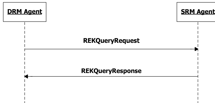
Figure 15: Sequence Diagram – REK Query
