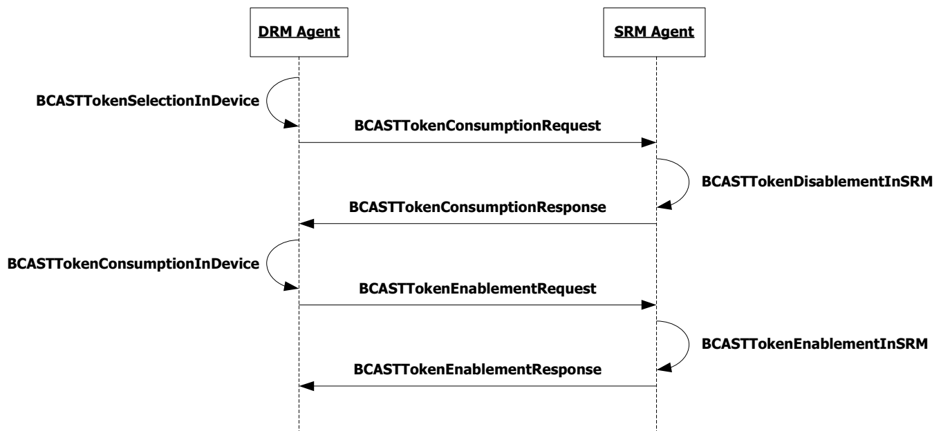
Figure 21: Sequence Diagram – Local BCAST Token Consumption
