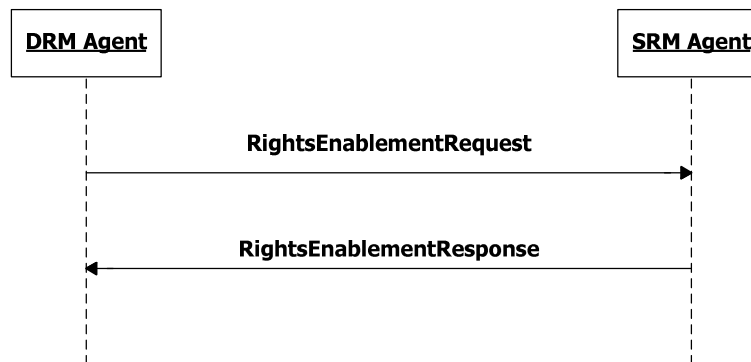
Figure 35: Sequence Diagram – Rights Enablement
