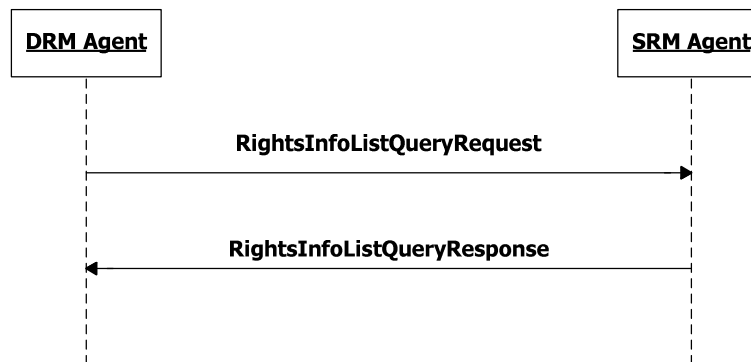
Figure 33: Sequence Diagram – Rights Information List Query
