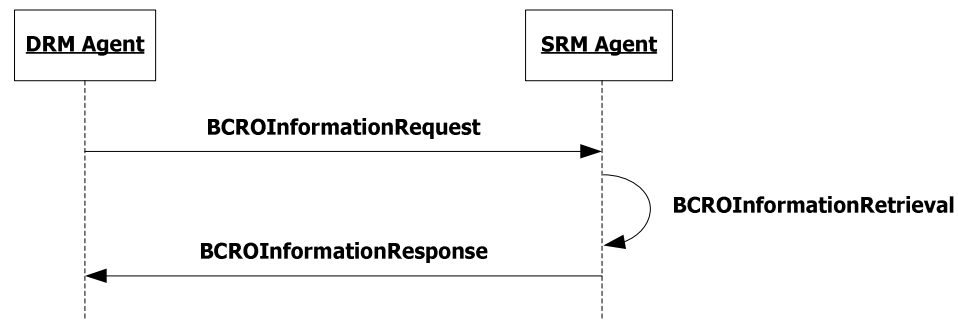
Figure 29: Sequence Diagram – BCRO Information Retrieval from SRM
