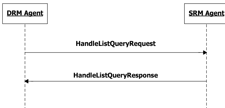
Figure 31: Sequence Diagram – Handle List Query
