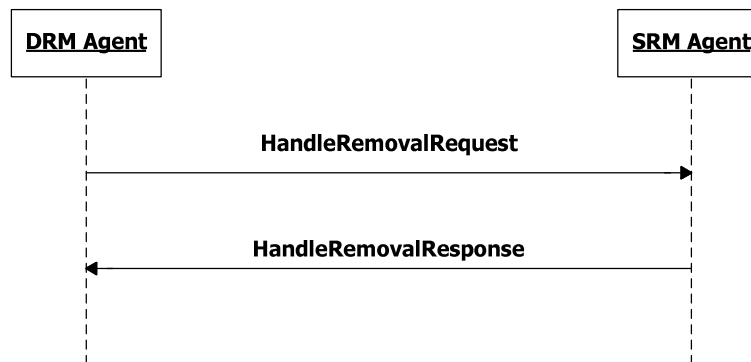
Figure 34: Sequence Diagram – Handle Removal
