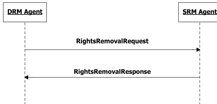
Figure 36: Sequence Diagram – Rights Removal
