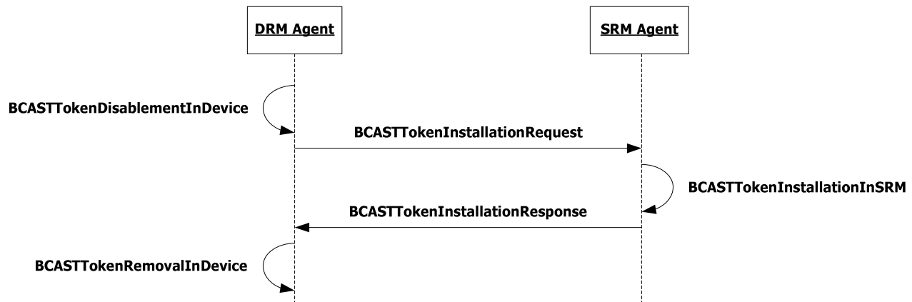
Figure 19: Sequence Diagram – BCAST Token Move from a Device to SRM
