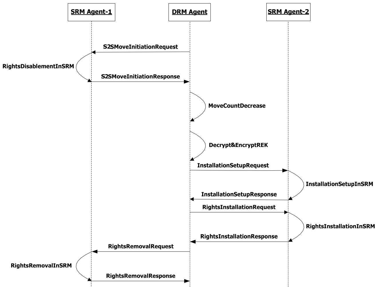
Figure 18: Sequence Diagram – SRM to SRM Move
