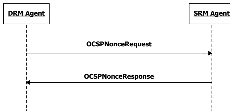
Figure 8: Sequence Diagram – OCSP Nonce
