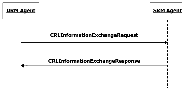
Figure 7: Sequence Diagram – CRL Information Exchange
