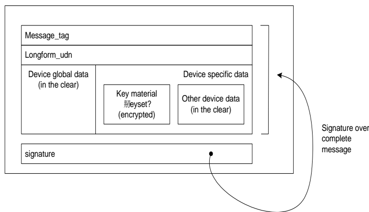
Figure 18: domain_registration_response() message
