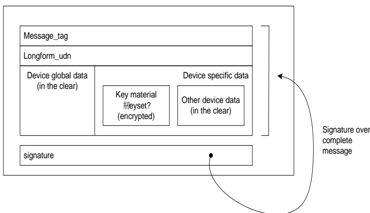
Figure 9: device_registration_response() message
