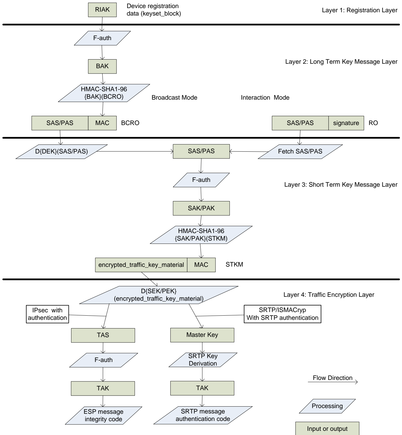
Figure 3: Authentication hierarchy
