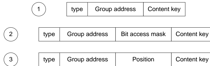
Figure 33: Addressing modes
