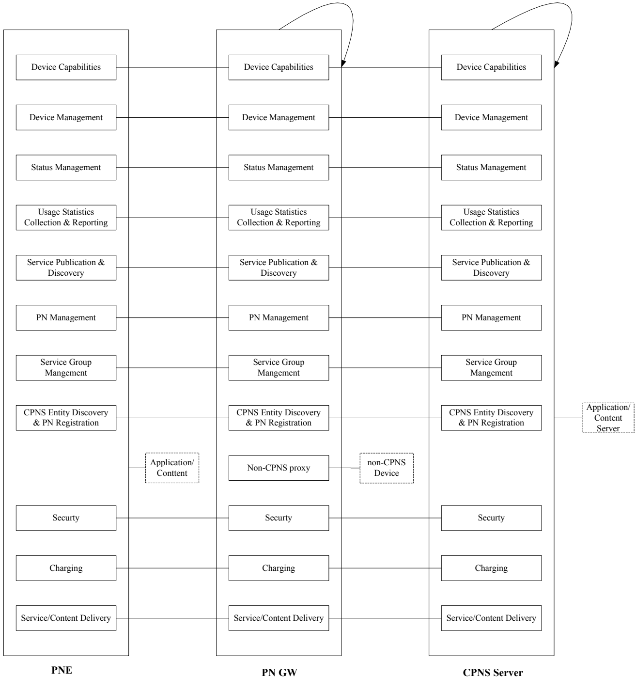
Figure 7: Functional diagram
