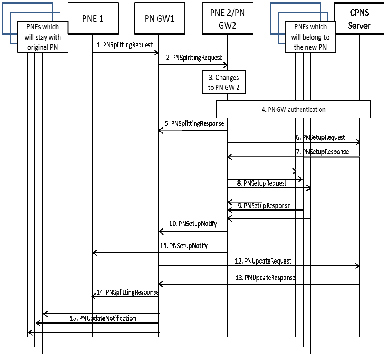
Figure 29 PN Splitting
