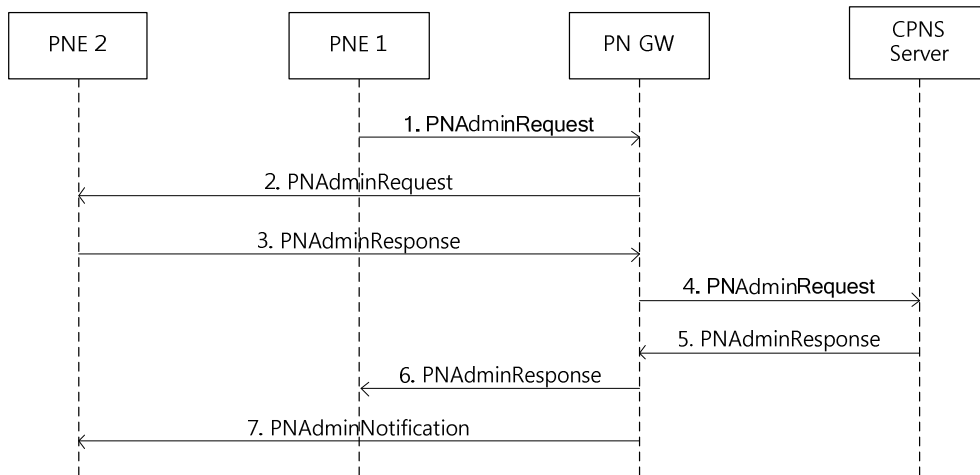
Figure 24 PNE requests Adminnee addition or removal
