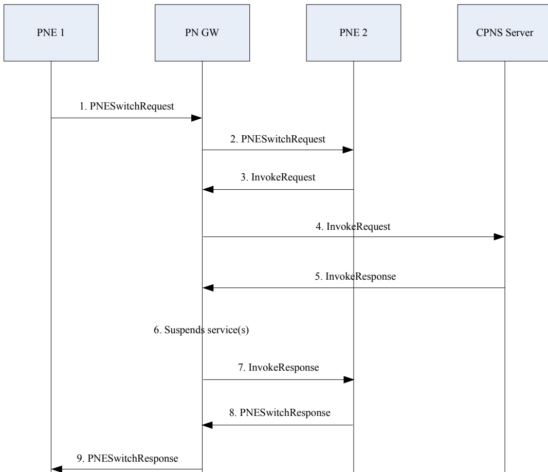
Figure 27 PNE Switching
