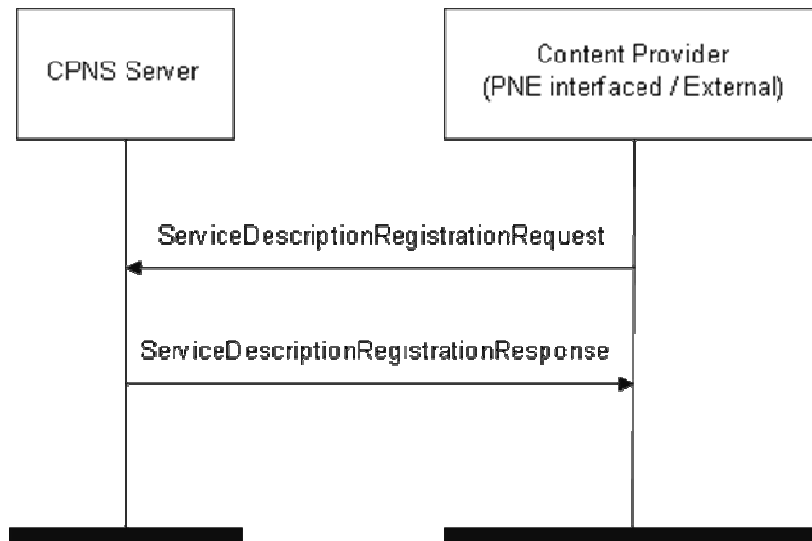
Figure 33 ServiceDescriptionRegistration flow
