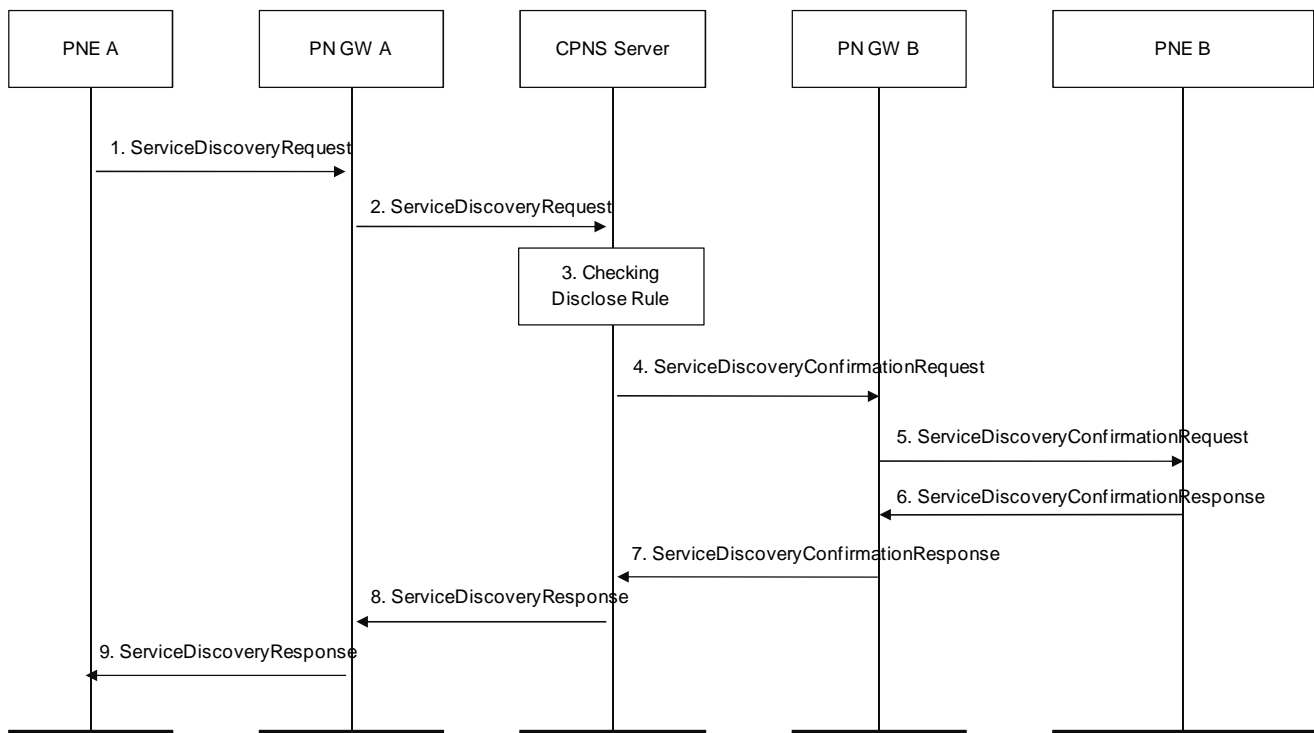
Figure 34 ServiceDiscoveryRequest/Response flow
