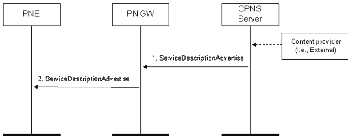
Figure 35 ServiceDescriptionAdvertise flow
