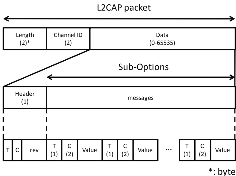
Figure 71 Bluetooth binding
