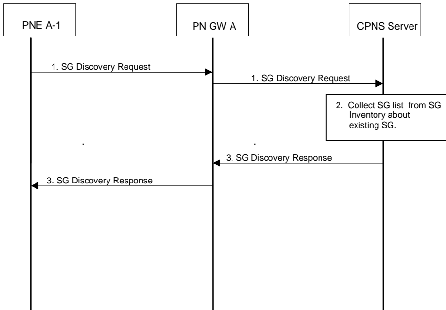
Figure 44 Flow of Service Group List Query
