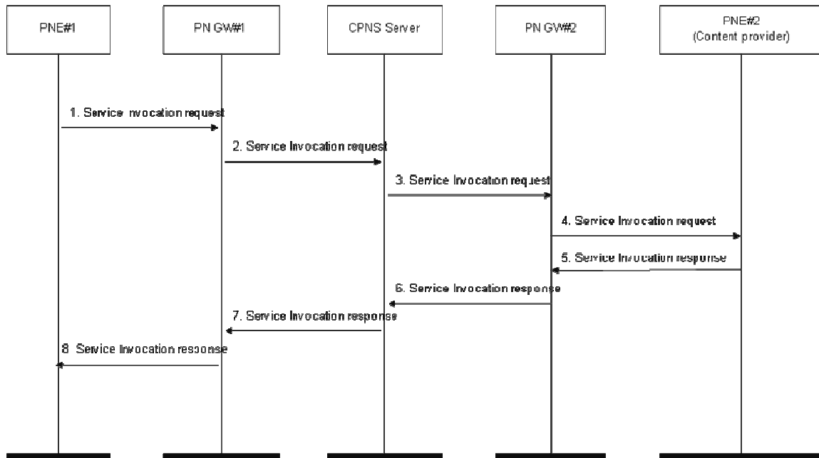
Figure 52 Service/Content Delivery flow-Remote PNE connection through CPNS Server
