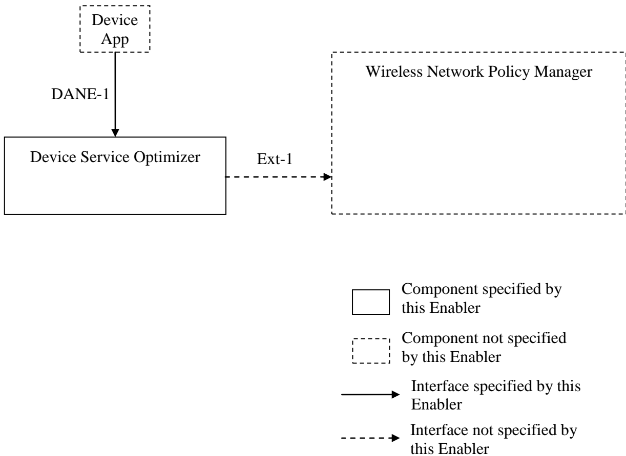
Figure 1: DANE Architectural Diagram
