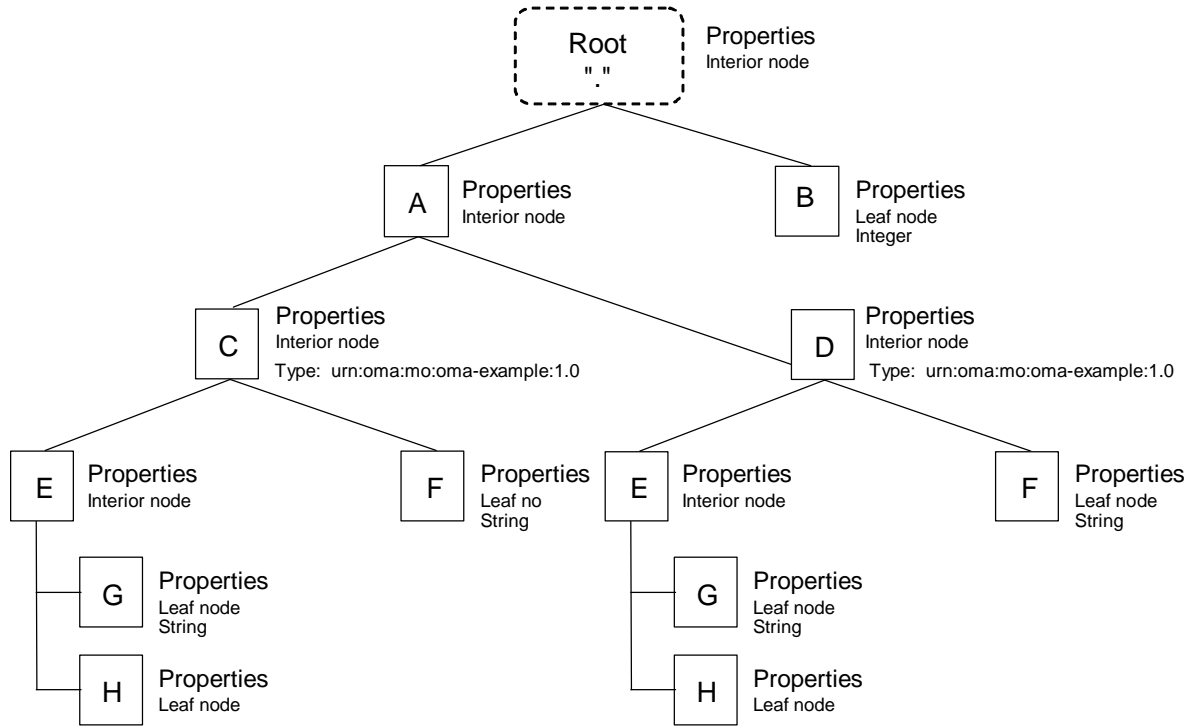
Figure 9: Example of Get with Attribute MORoot
