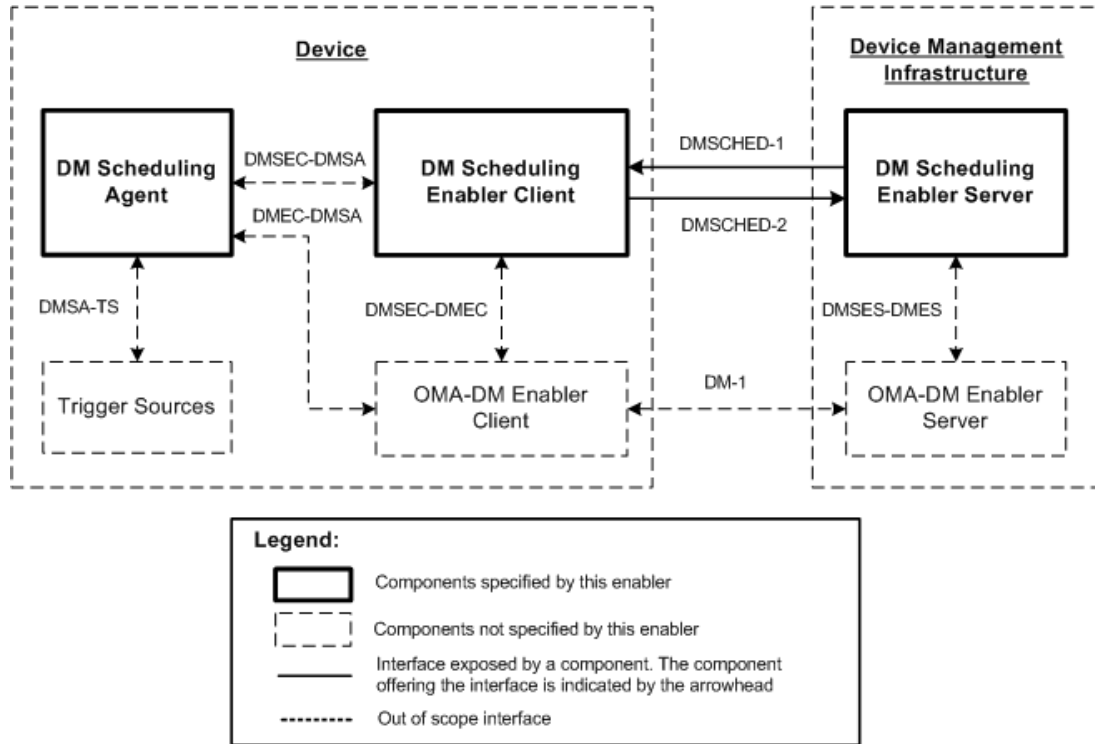
Figure 2: Device Management Scheduling Framework Architecture
