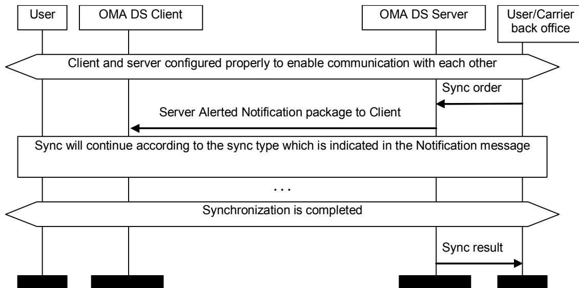
Figure 11 MSC of the Server Alerted Sync session
