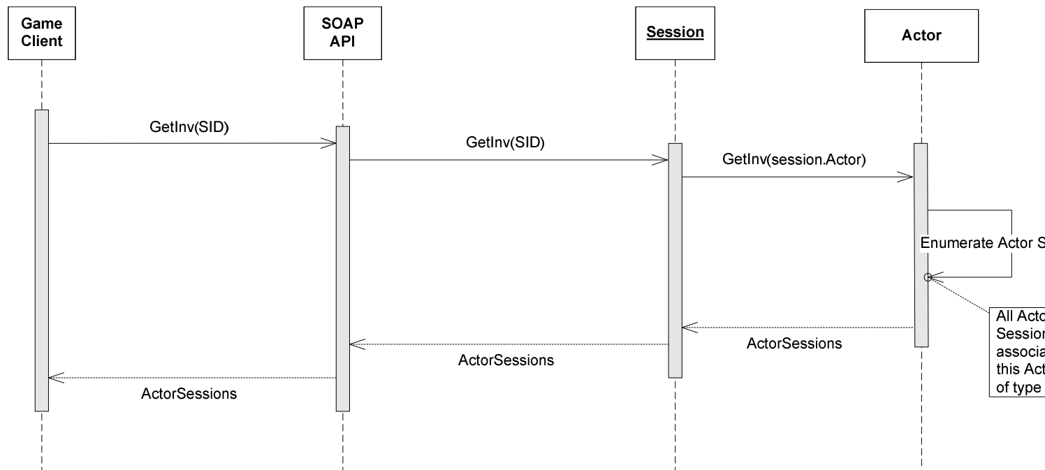
Figure 7: Get invitation operation
