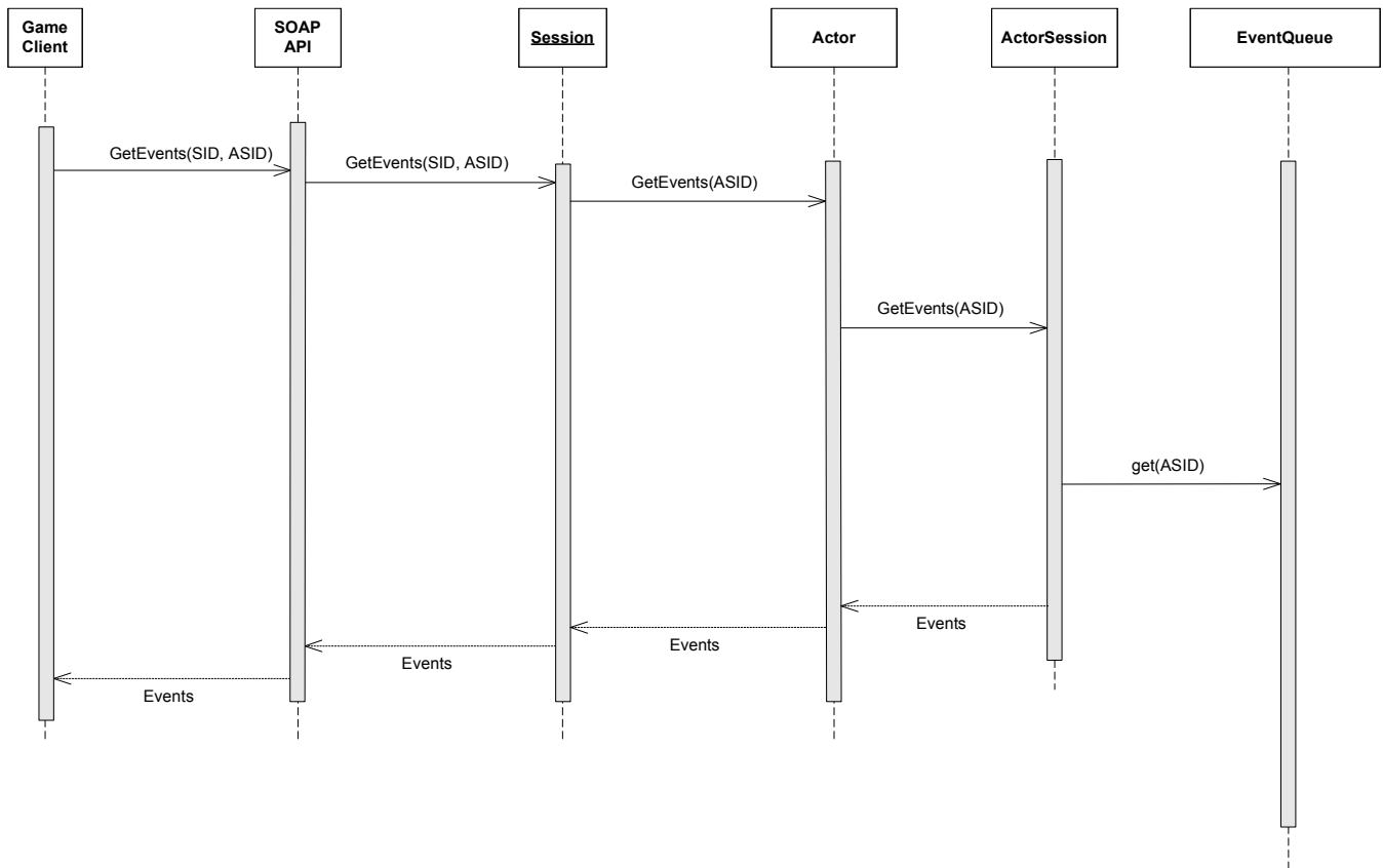
Figure 30: Get Event Operation
