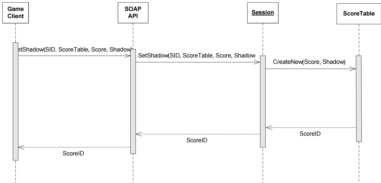
Figure 25: Set Shadow Operation
