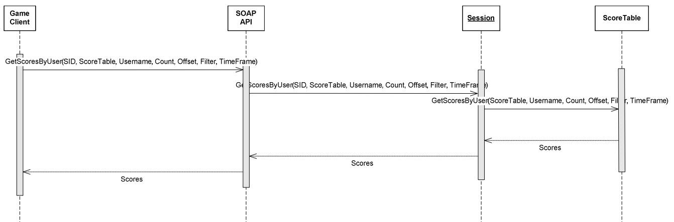
Figure 24: Get a certain number of scores for a specific user name Operation
