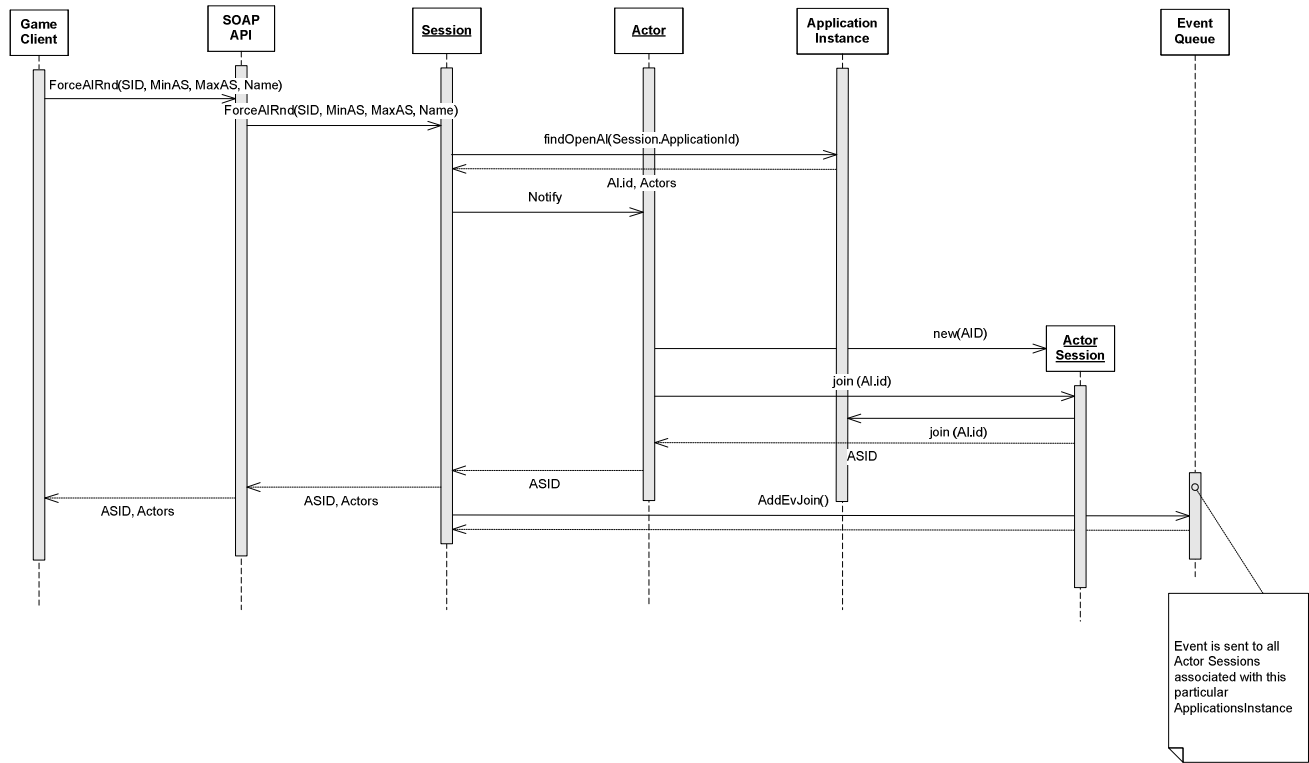
Figure 13: Actor joins a randomly selected Application instance operation
