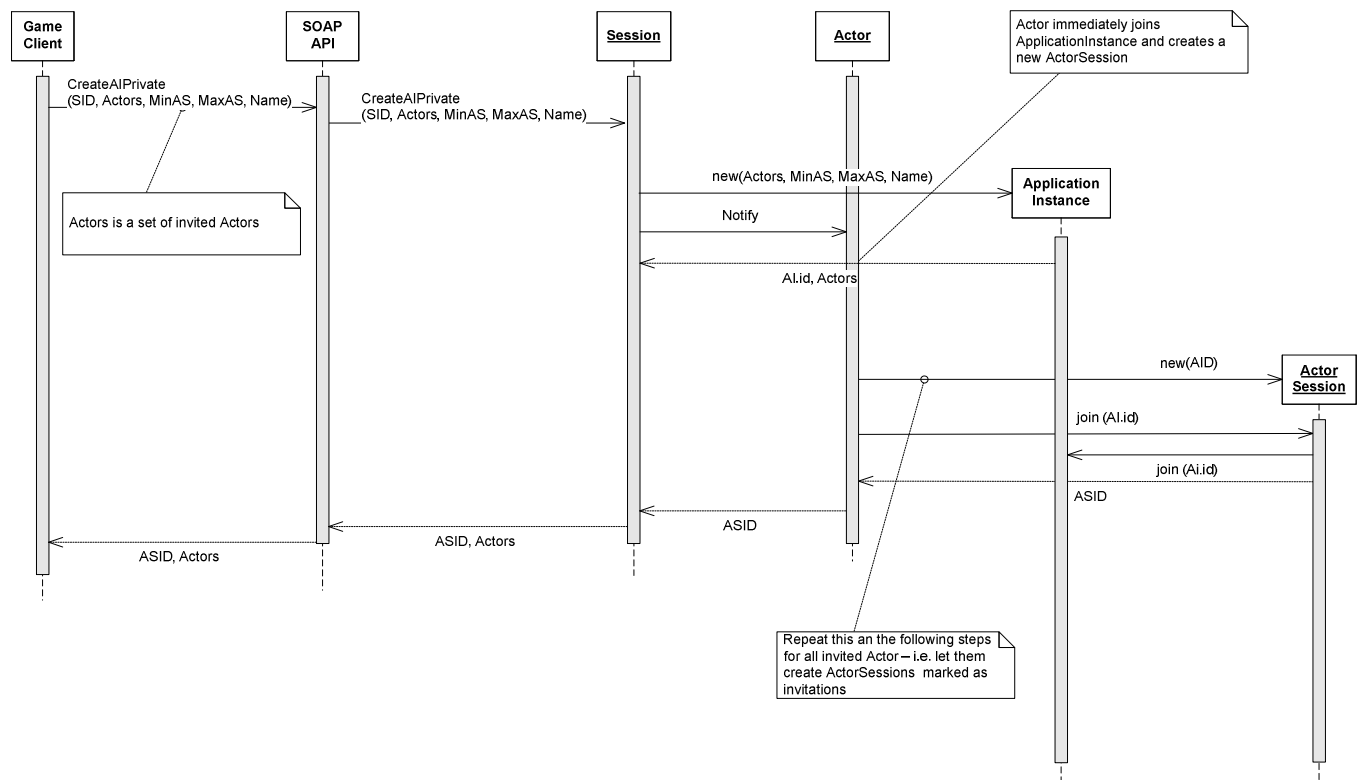
Figure 12: Create a Private Application instance operation
