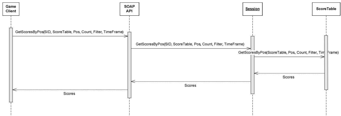
Figure 22: Retrieve a certain number of scores from a position operation
