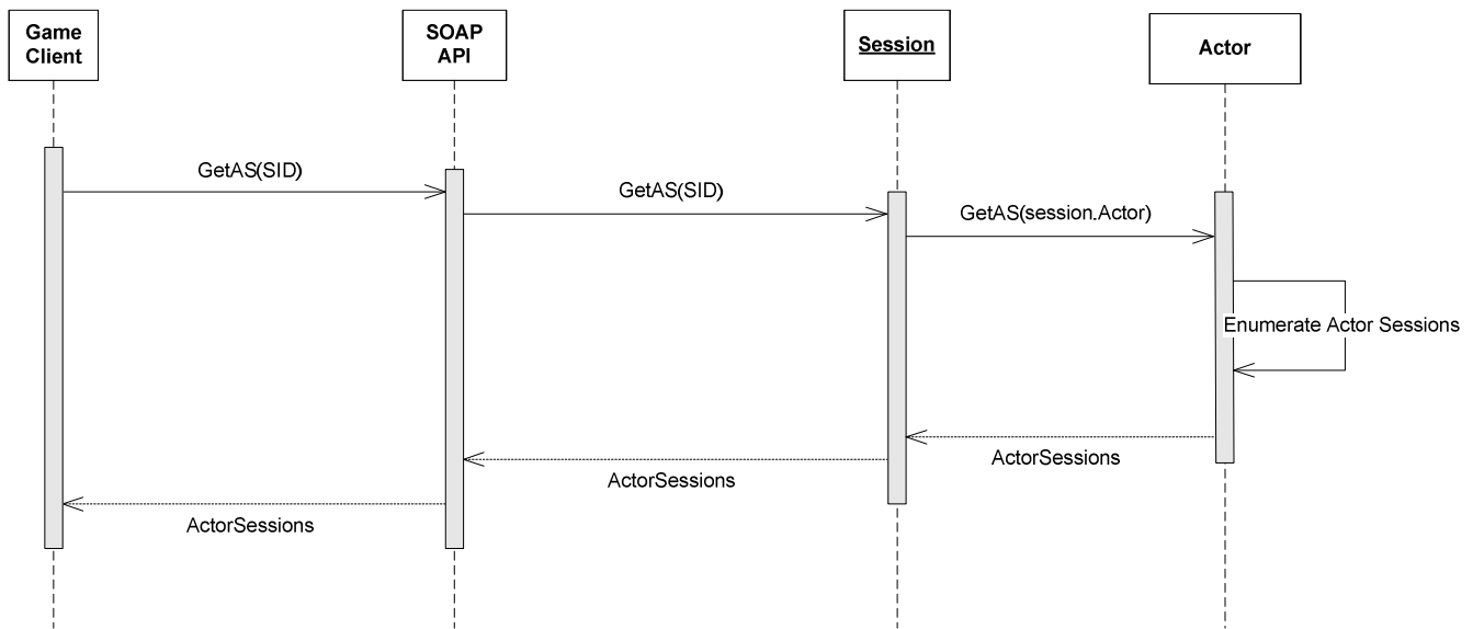
Figure 6: Get Actor Session operation
