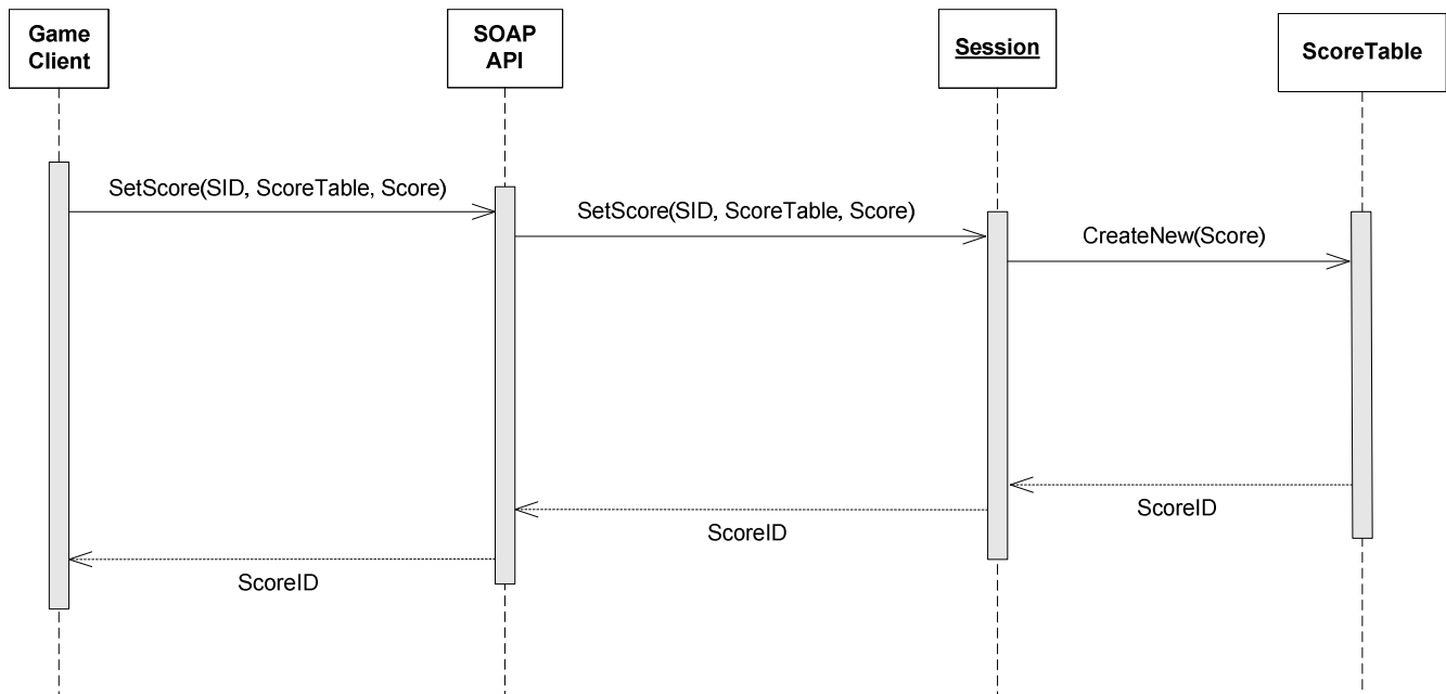
Figure 20: Set Score operation
