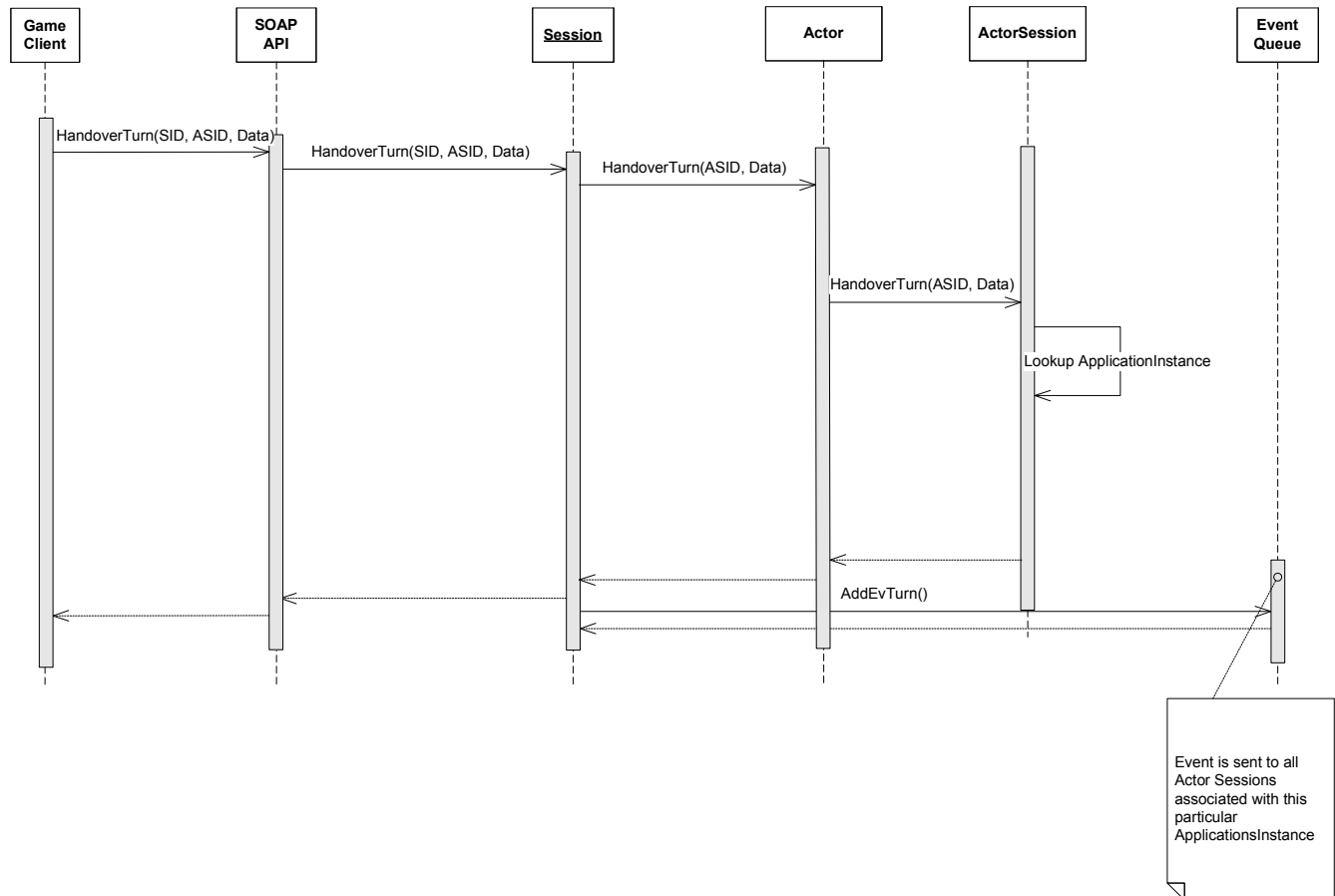
Figure 17: Handover Turn operation
