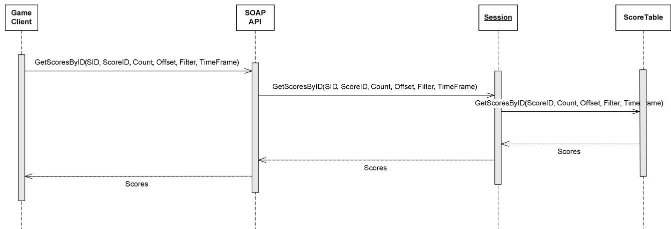
Figure 23: Retrieve a certain number of scores for a certain ID Operation
