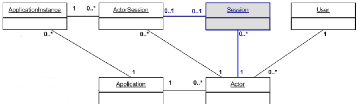
Figure 2: The server side Domain model
