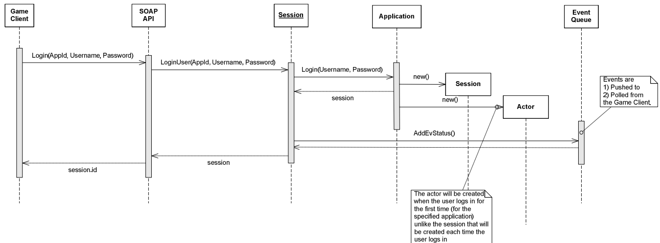
Figure 3: Login Operation (App User)
