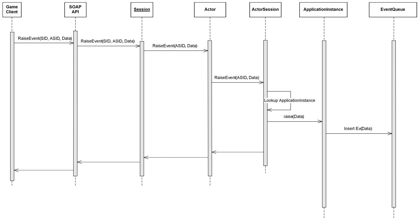
Figure 32: Raise Event Operation
