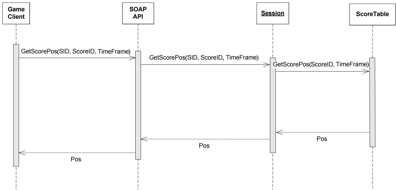
Figure 21: Get a position for the score Operation
