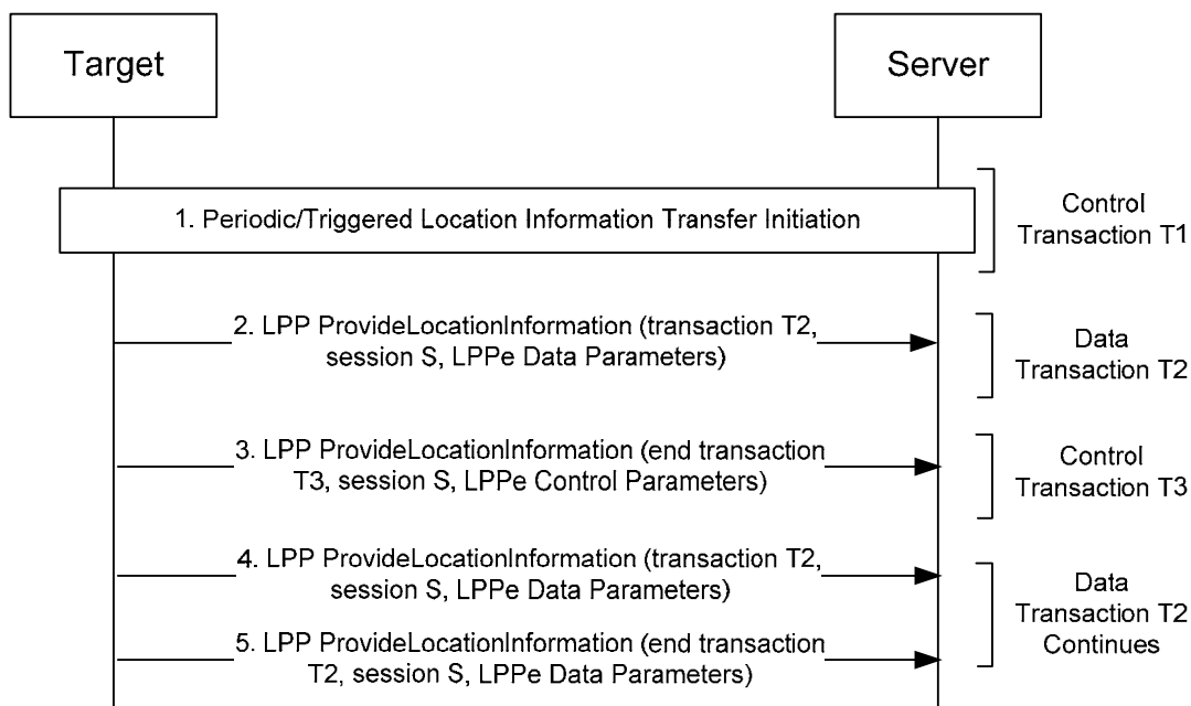
Figure 6 : LPPE Periodic/Triggered Location Information transfer procedure with Target Update
