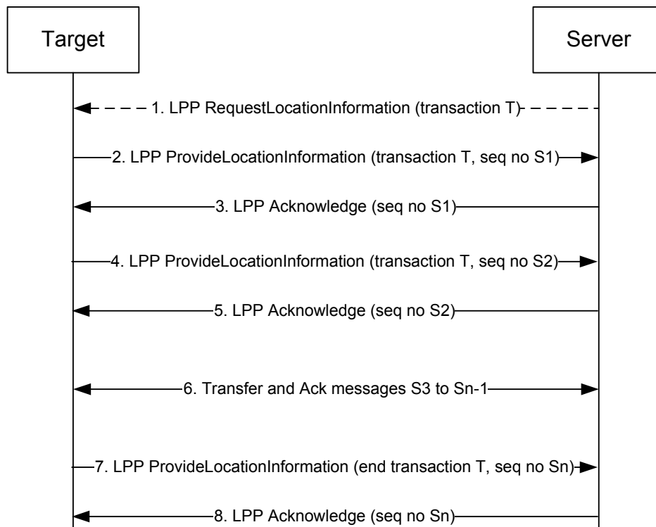
Figure 9: LPPE Segmented Location Information Transfer
