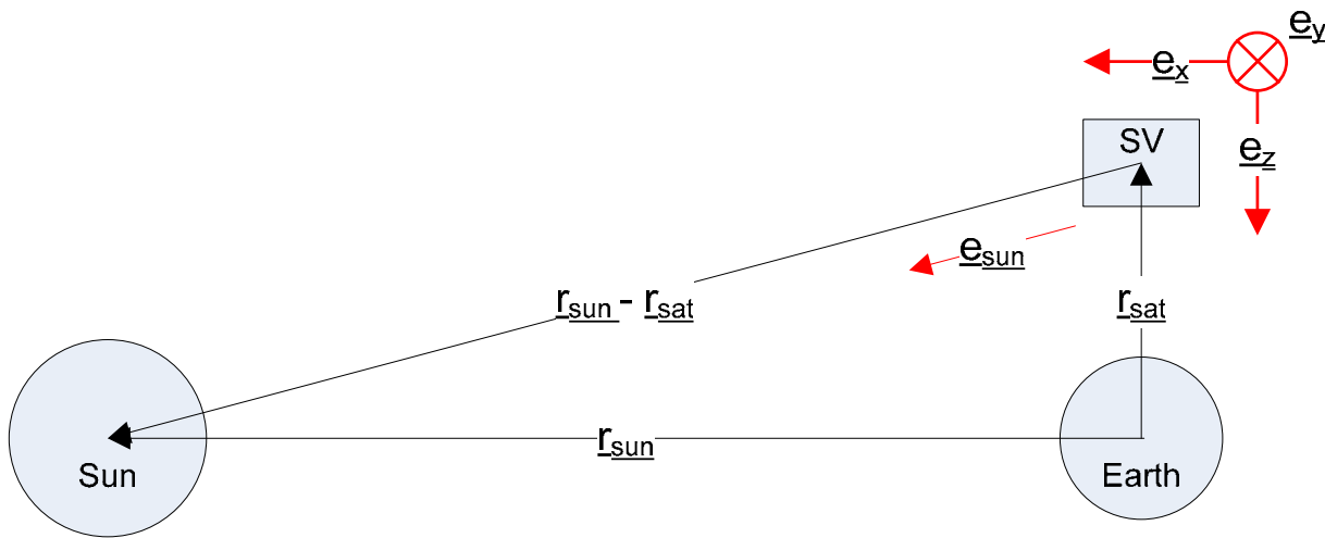
Figure 14: Satellite-fixed coordinate system
