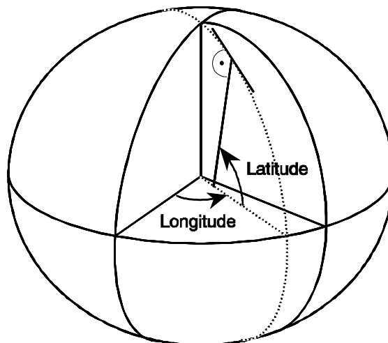
Figure 12: Ellipsoid Coordinates
