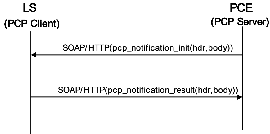
Figure 4: SOAP/HTTP sequence for PCPNotificationService
