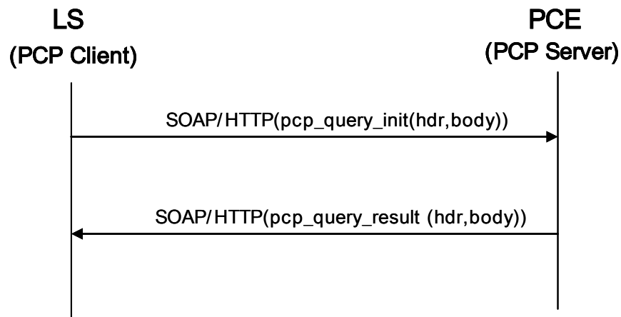
Figure 3: SOAP/HTTP sequence for PCPQueryservice
