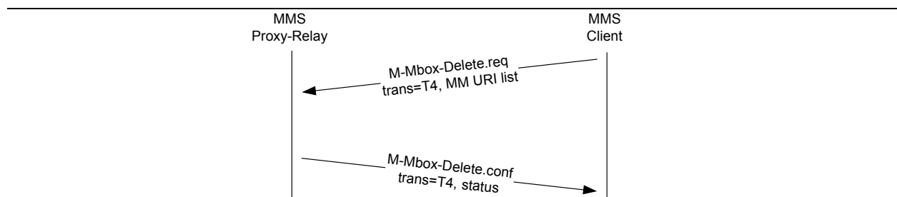
Figure 20. Example MMS Delete from MMBox Transaction
