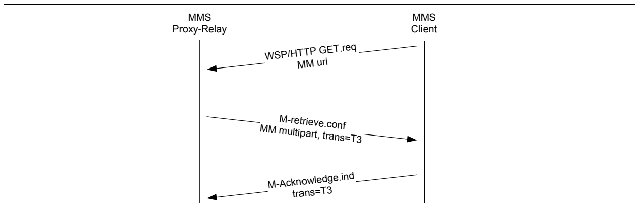
Figure 12. Example MMS Retrieval Transaction with Acknowledgement
