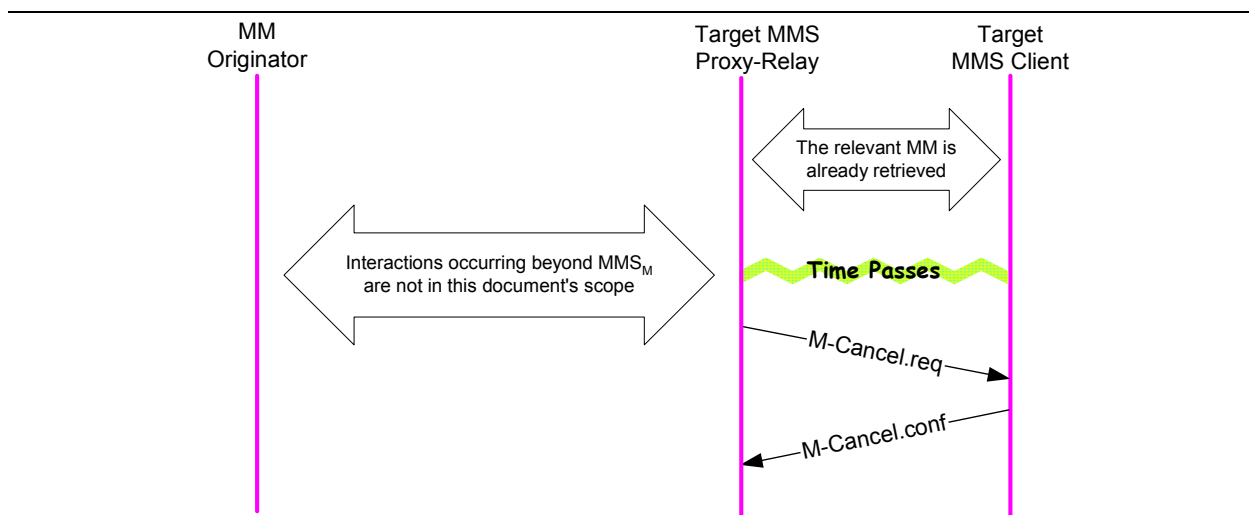
Figure 9: Example MMS M Transaction Flow – Cancel an already retrieved MM
