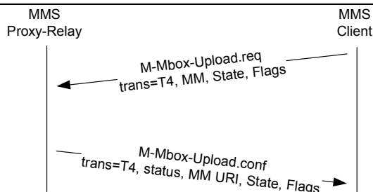
Figure 23: Example MMS Upload to MMBox Transaction
