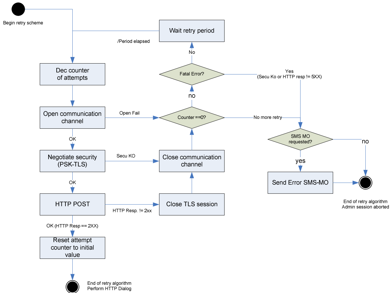
Figure 3: Retry algorithm
